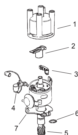
Bosch Distributor
