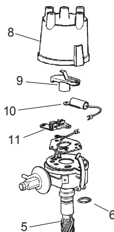
Motorcraft Distributor
