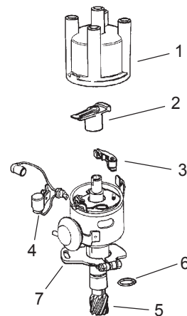
Bosch Distributor
