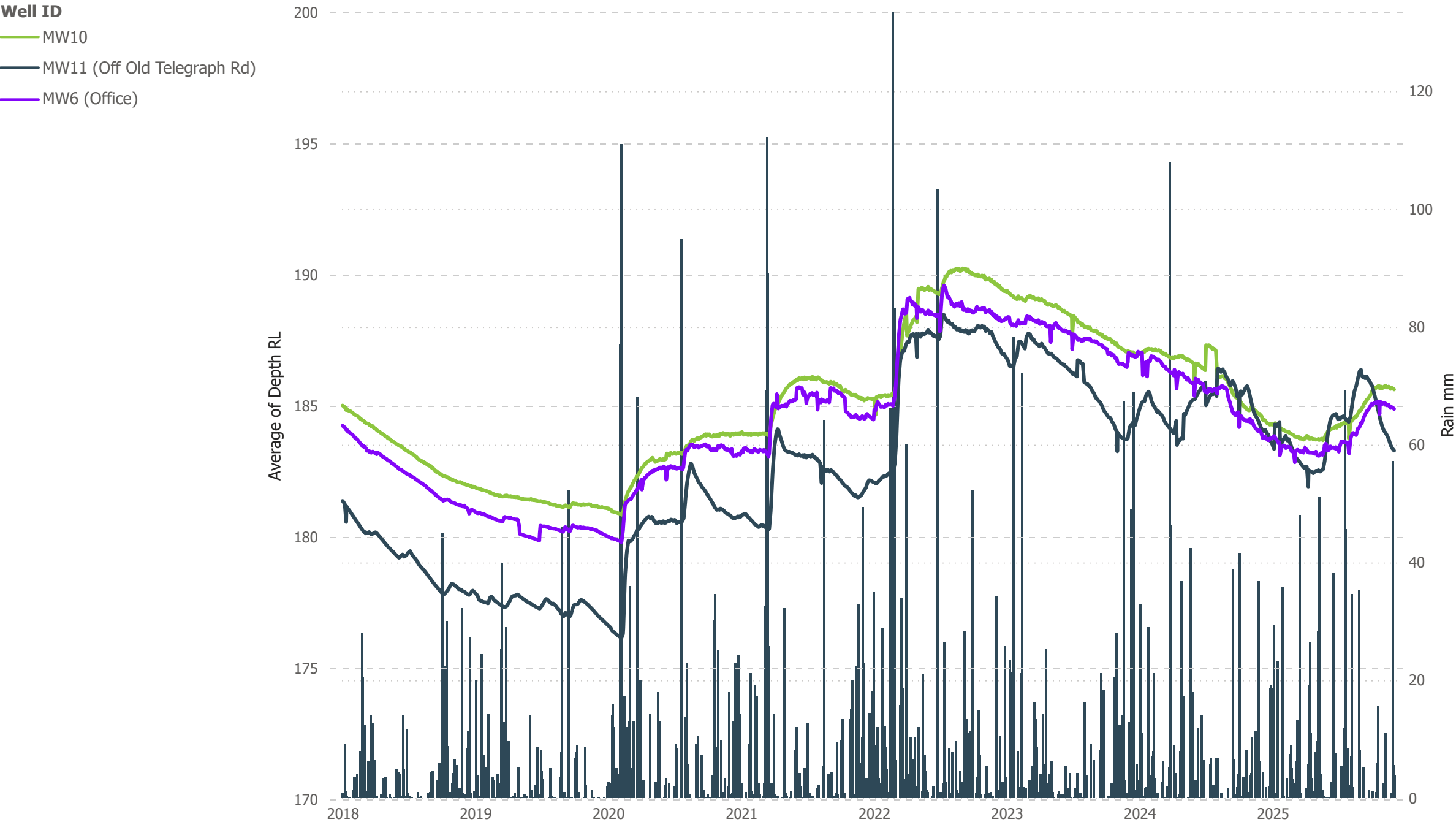
Graph 3: All Groundwater Depths with Rainfall in Maroota Sand
