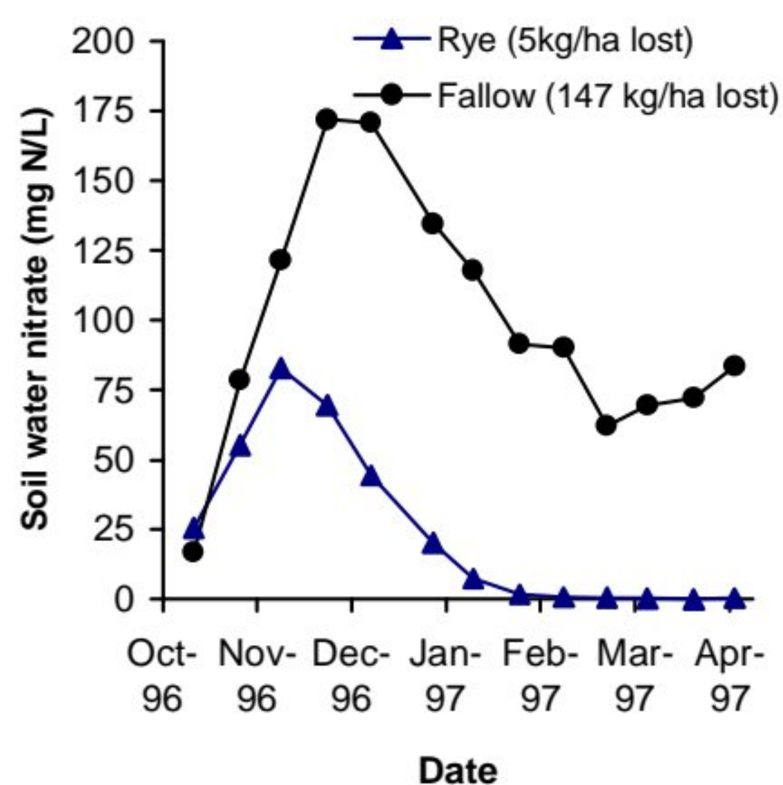
Figure 1. An example of overwinter nitrate concentrations below bare soil plots and plots on which grazing rye was growing. This trial was set up directly after the incorporation of a grass/clover ley.
