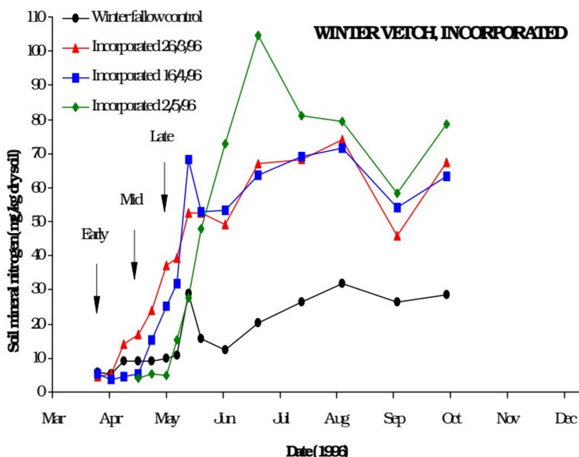
Figure 2. An example of patterns of soil mineral nitrogen (0-30cm) after incorporation of an overwintered vetch crop at three different dates in the spring
