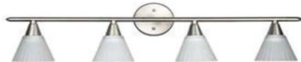
aa: 114 VS114-3100BN W33-1/2"*H8-1/2" *6" 4*E26*100W BN/ WH OPAL
