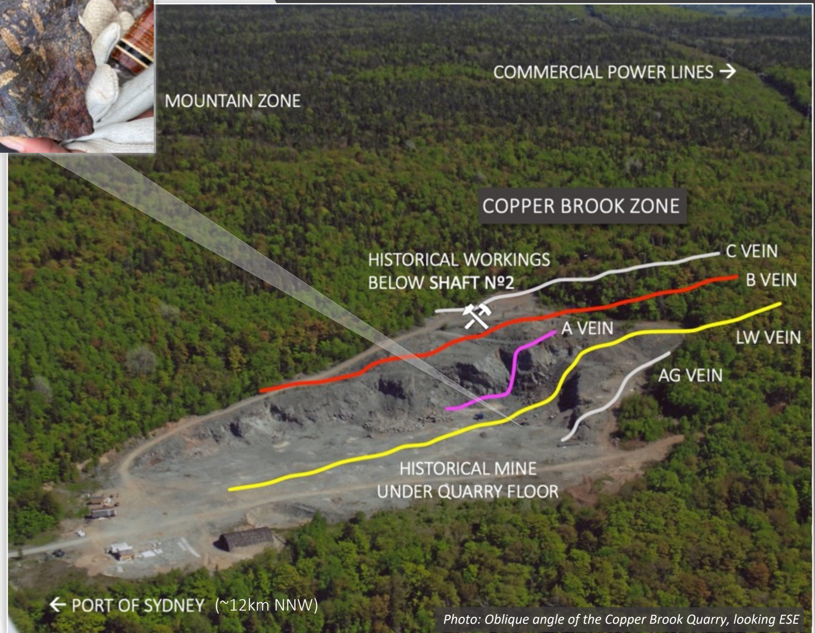
MINERALIZED TOURMALINE BRECCIA
