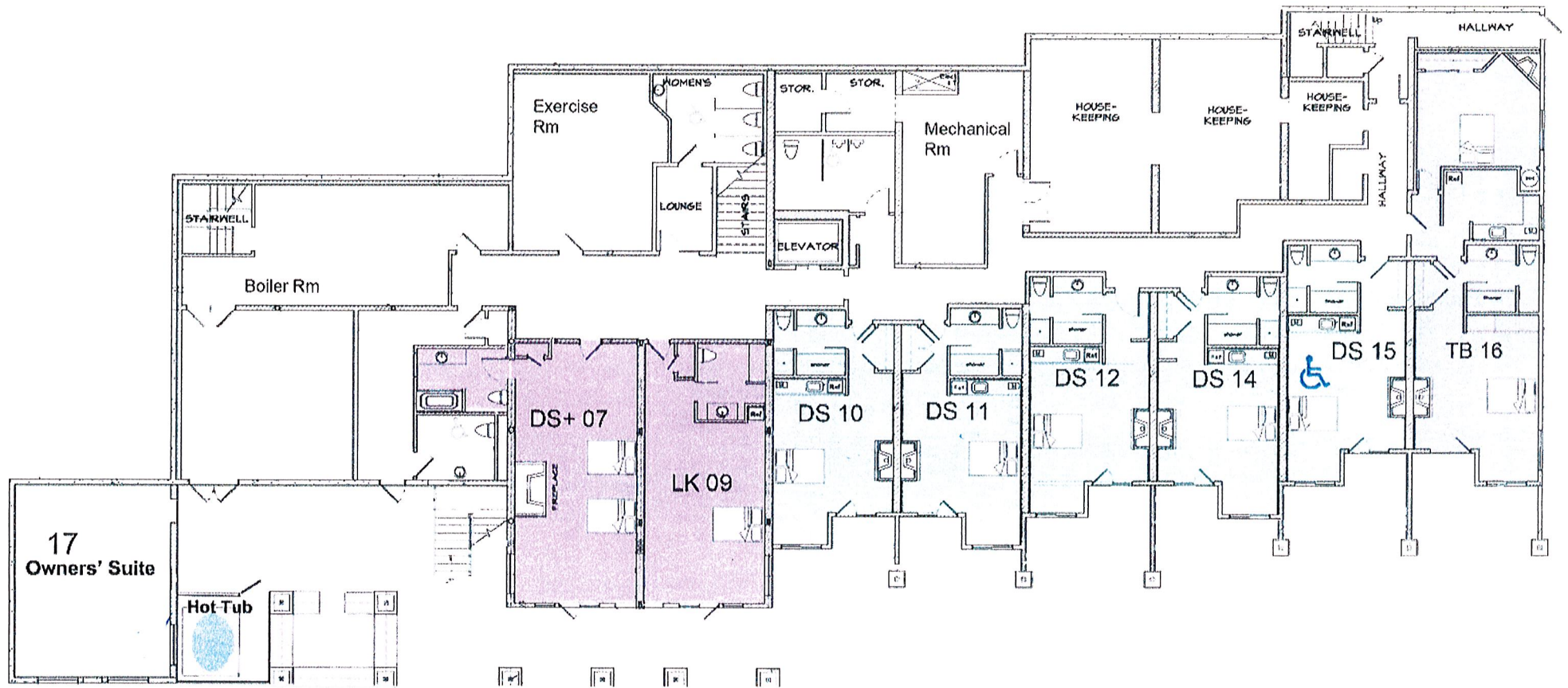
Lodge Floorplan Level 1 (Lake Level)
