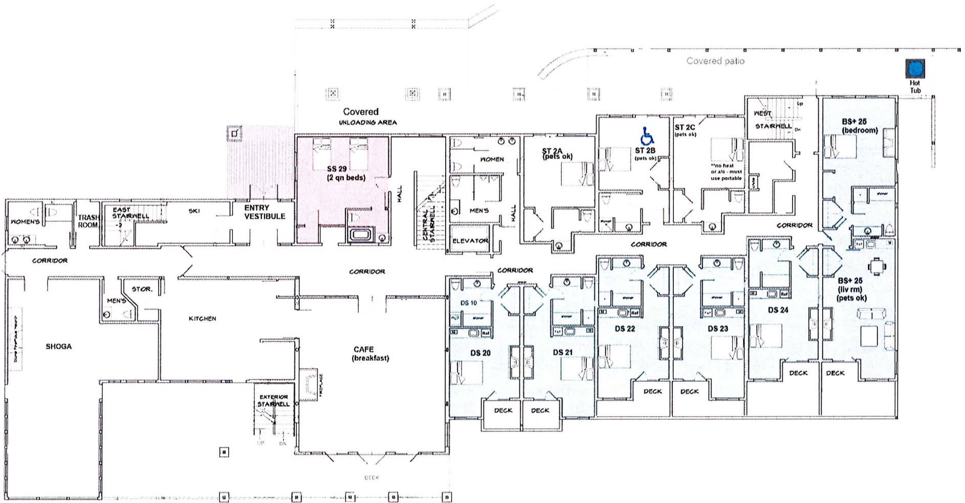
Lodge Floor Plan Level 2
