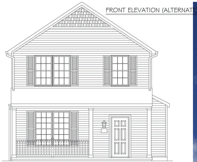
FRONT ELEVATION A
