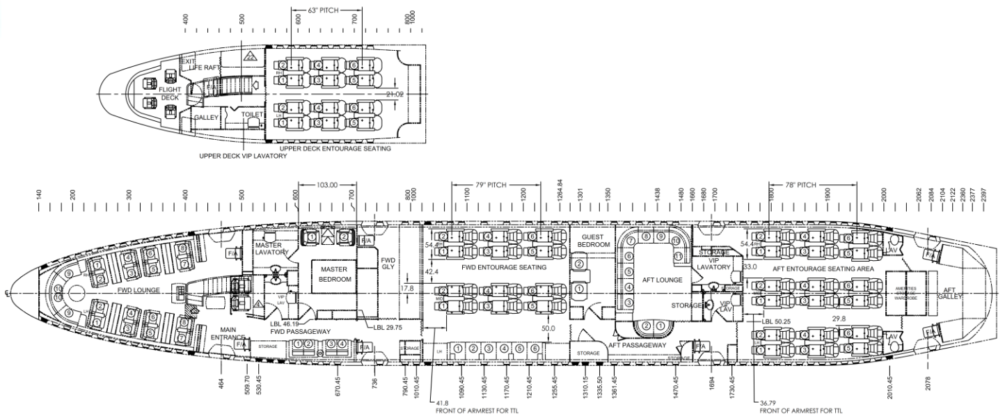
Interior Layout of Boeing 747SP
