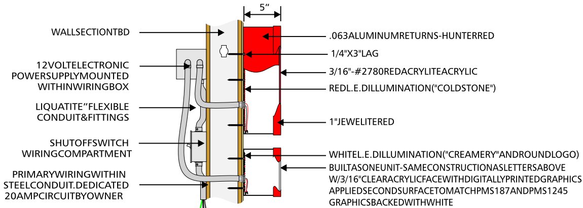
COLD STONE CREAMERY CHANNEL LETTER SECTION VIEW Not to scale
