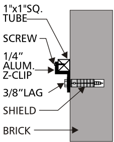
MOUNTING TYPE "B" TOP VIEW OF TRUSS SCALE: 1.5" = 1'
