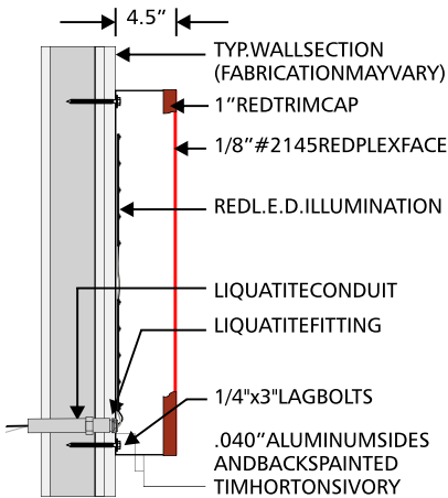
TIM HORTONS CHANNEL LETTER SECTION VIEW Not to scale
