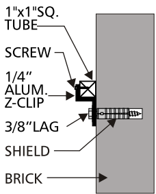
MOUNTING TYPE "A" SIDE VIEW OF TOP BAR SCALE: 1.5" = 1'
