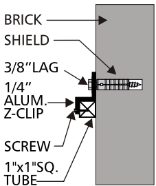
MOUNTING TYPE "C" SIDE VIEW OF BOTTOM BAR SCALE: 1.5" = 1'
