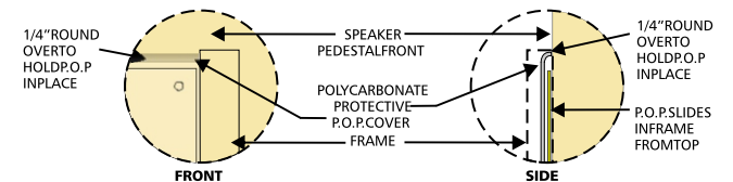
PROTECTIVE P.O.P. COVER DETAIL
