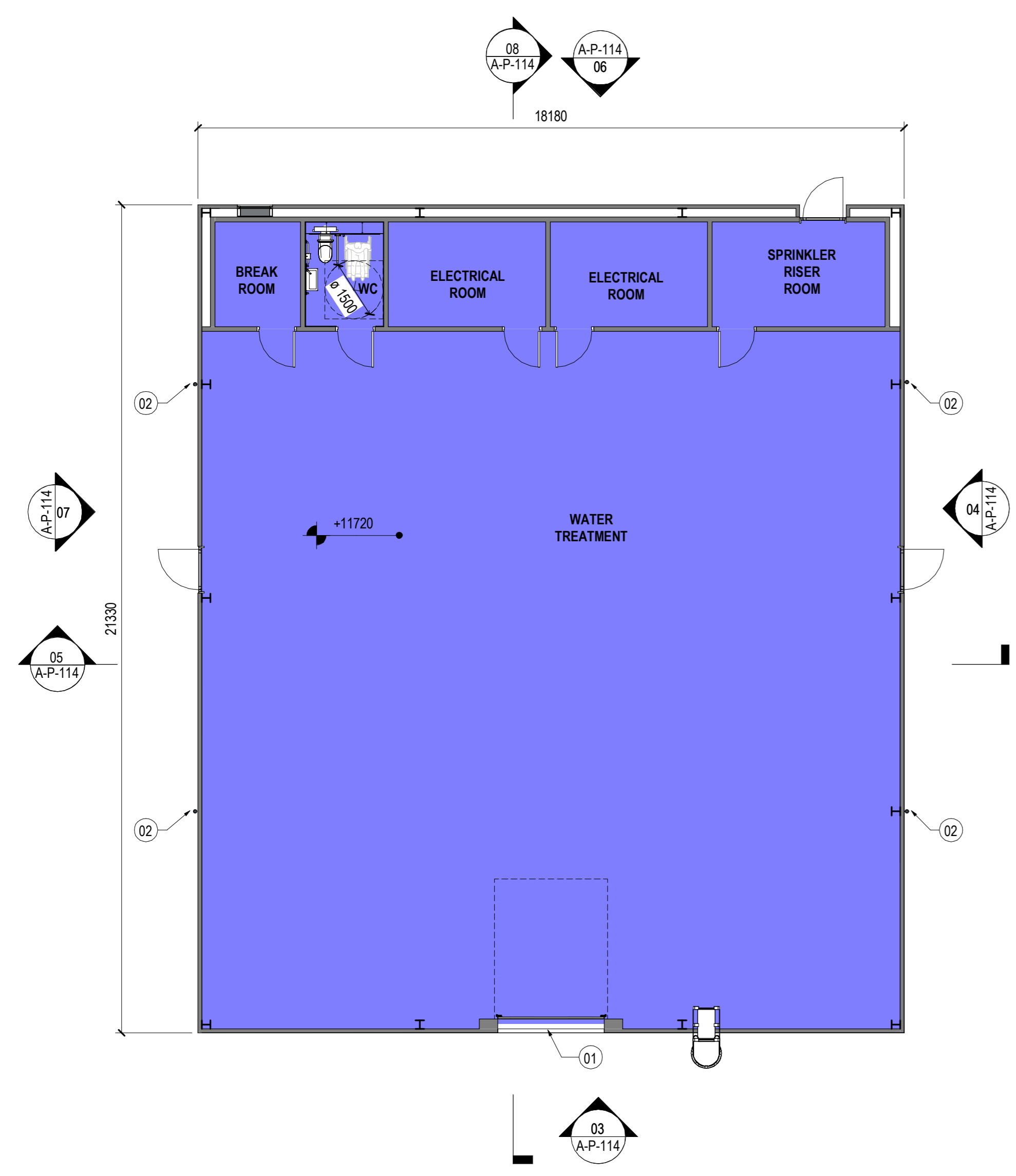
01 WATER TREATMENT BUILDING - FLOOR PLAN SCALE: 1:100
