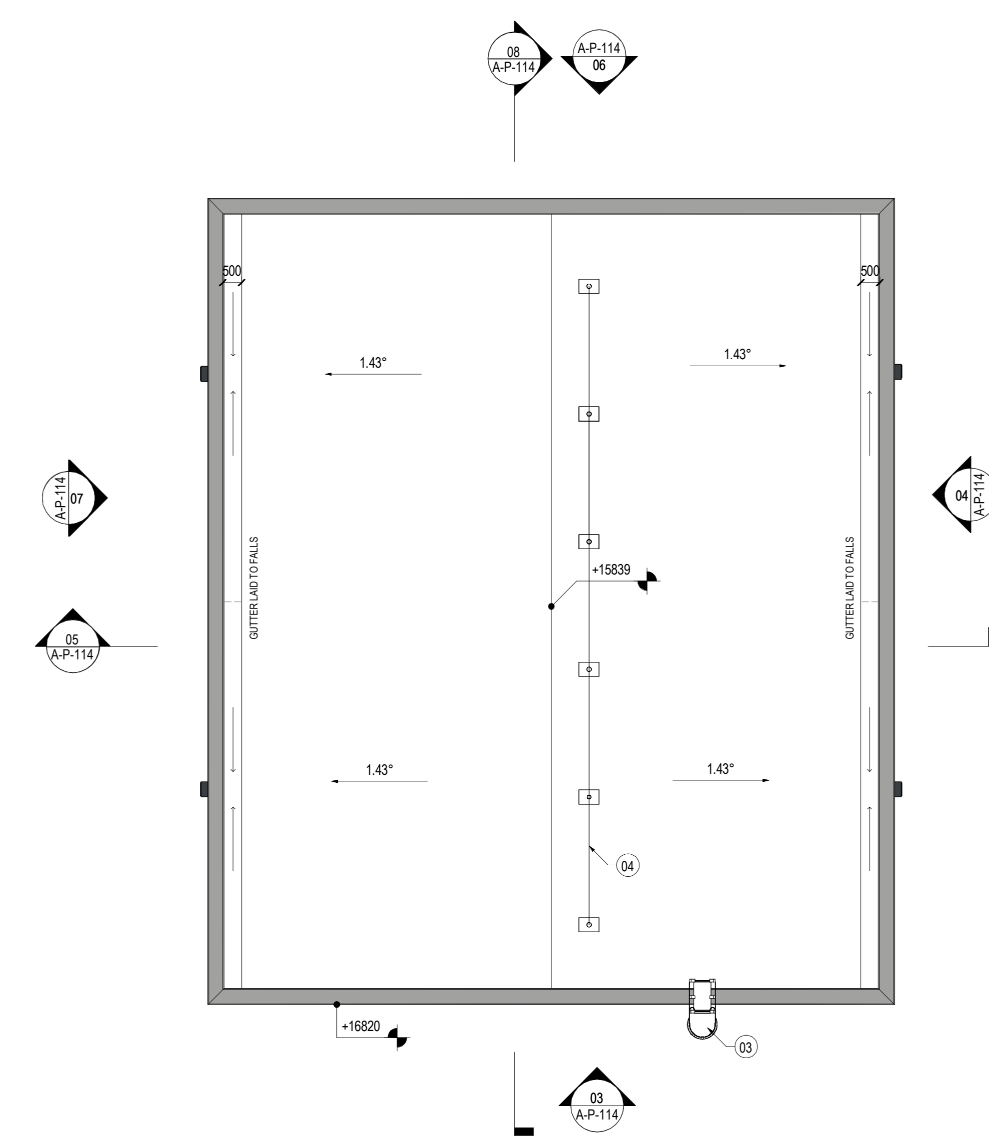
02 WATER TREATMENT BUILDING - ROOF PLAN SCALE: 1:100
