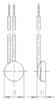
Installation height h from 3,4 mm Diameter d 9,0 mm
