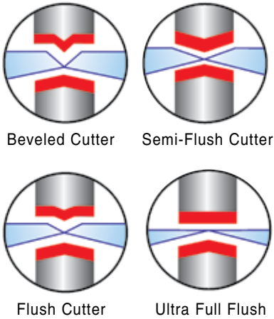
Flush Cutter
