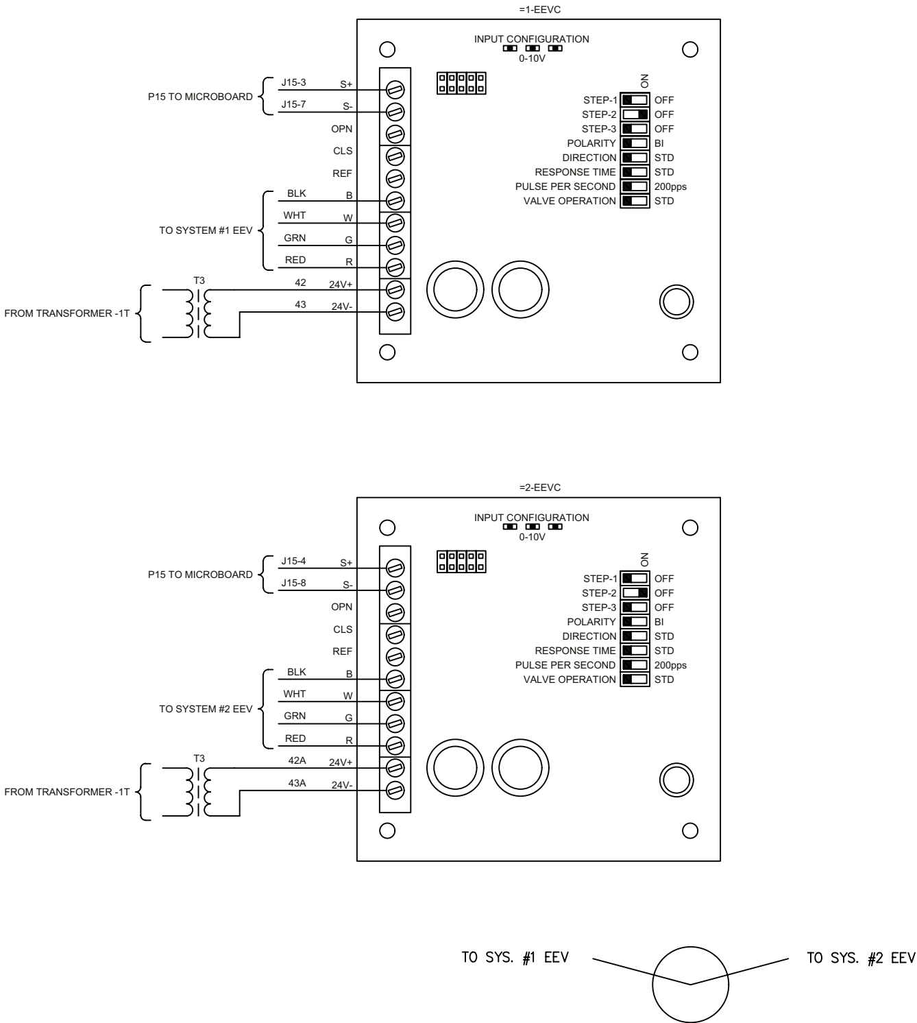
FIGURE 22 - EEV CONTROLLER ELEMENTARY DIAGRAM
