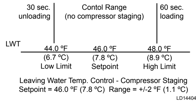
FIGURE 46 - LEAVING WATER TEMPERATURE CONTROL EXAMPLE
