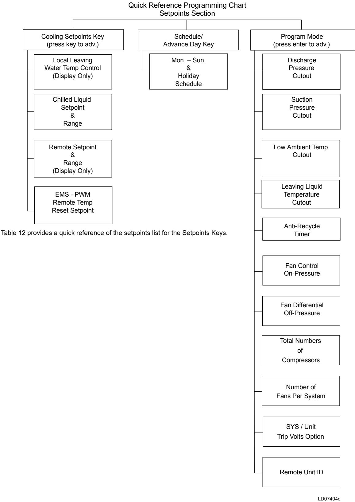
FIGURE 43 - SETPOINTS QUICK REFERENCE LIST
