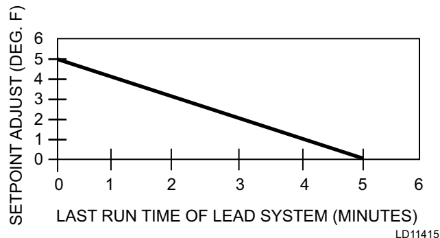
FIGURE 47 - SETPOINT ADJUST
