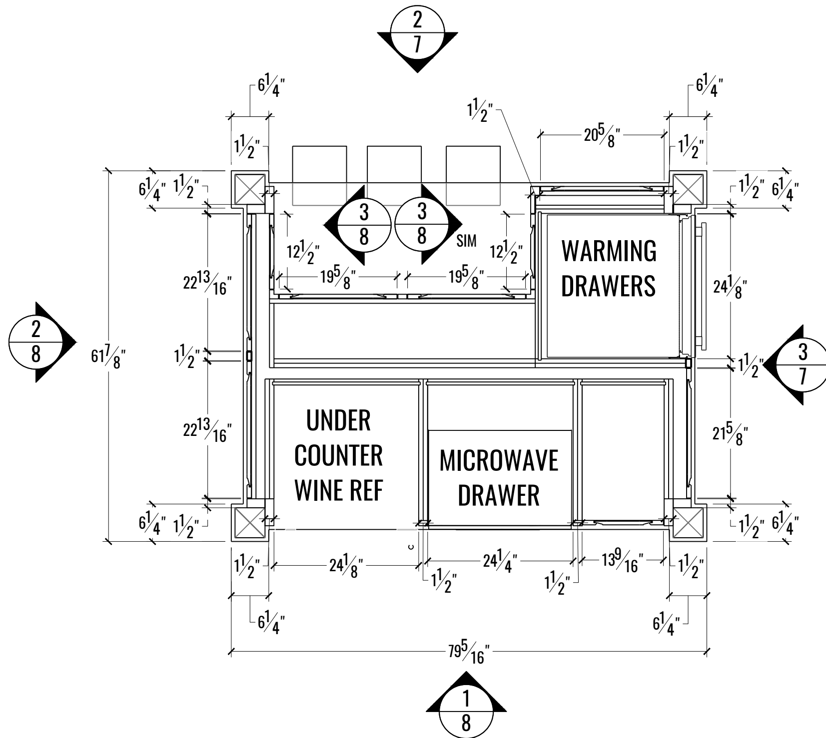
1 PLAN: KITCHEN ISLAND SCALE: 3/4" = 1'-0"
