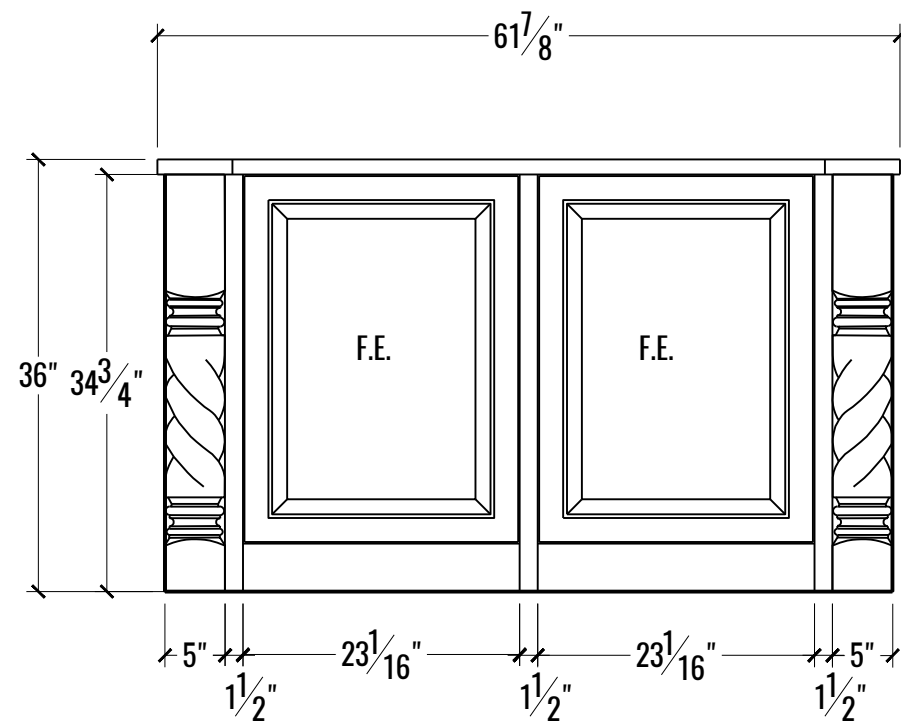
2 8 ELEVATION: ISLAND FINISHED END SCALE: 3/4" = 1' - 0"
