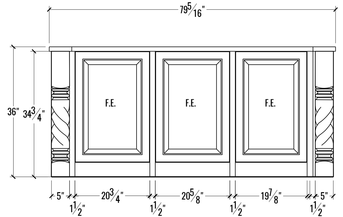
2 ELEVATION: ISLAND SEATING SIDE SCALE: 3/4" = 1'-0"
