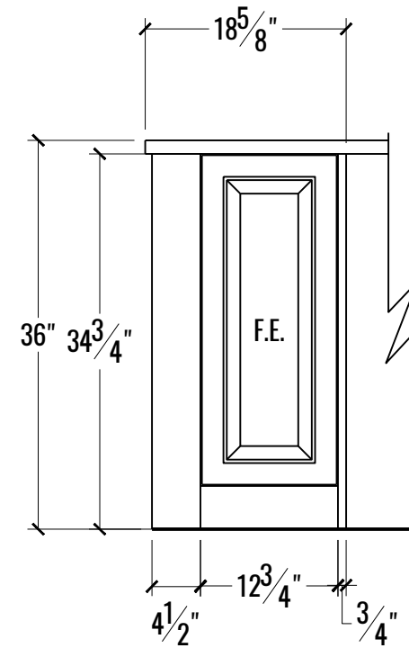
3 8 ELEVATION: ISLAND SEATING SIDE FINISHED END (SIDE) SCALE: 3/4" = 1' - 0"
