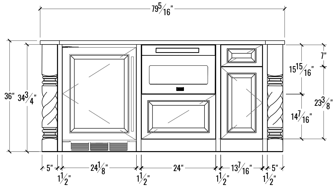
1 8 ELEVATION: ISLAND UNDERCOUNTER WINE REFRIGERATOR SCALE: 3/4" = 1' - 0"
