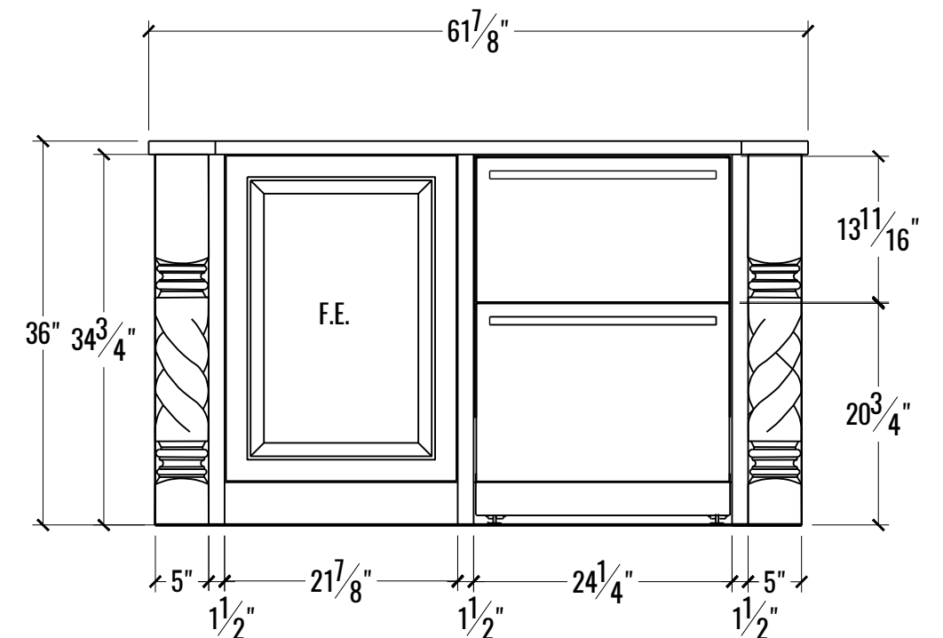
3 ELEVATION: ISLAND WARMING DRAWER SIDE SCALE: 3/4" = 1'-0"
