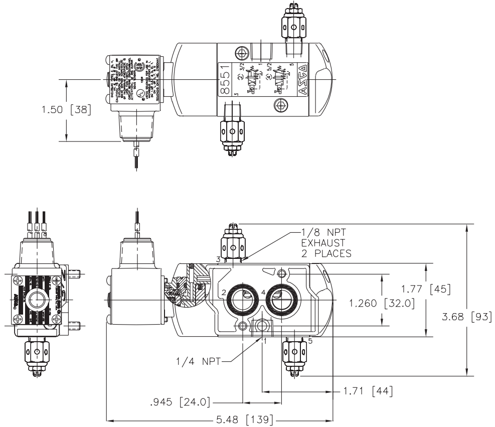
Constr. Ref. 2
