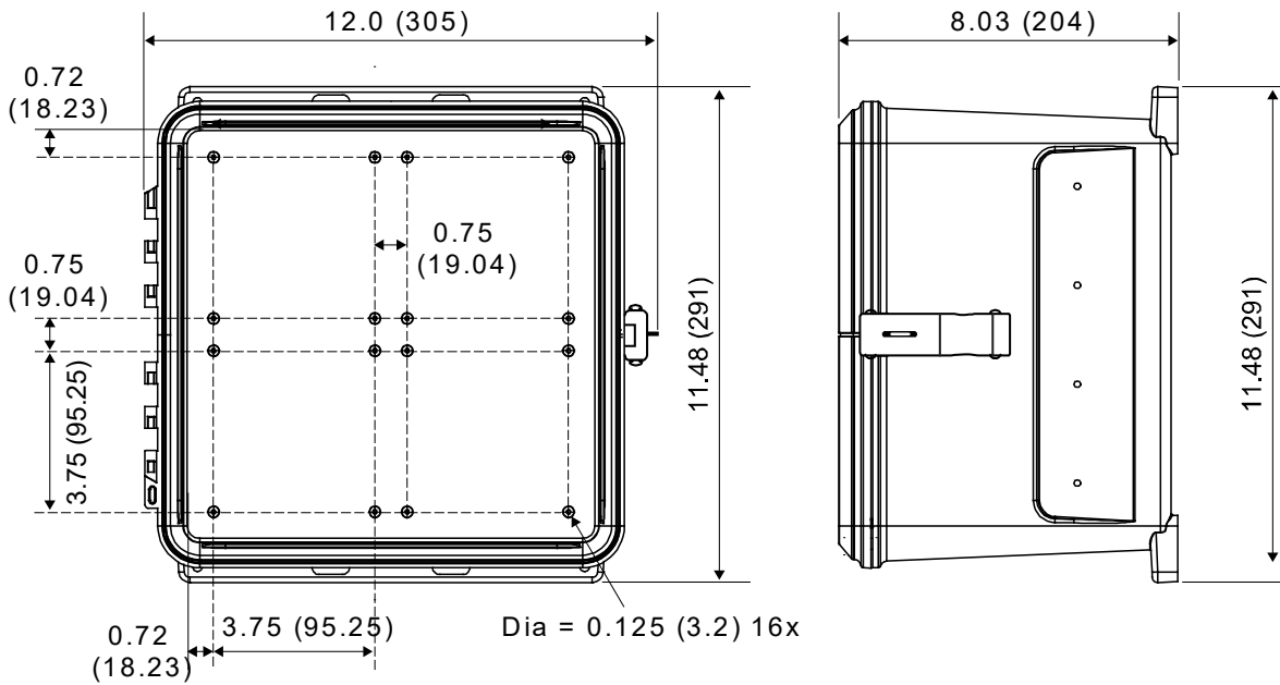
Figure 7. Wall Mount & Internal Boss Dimensions
