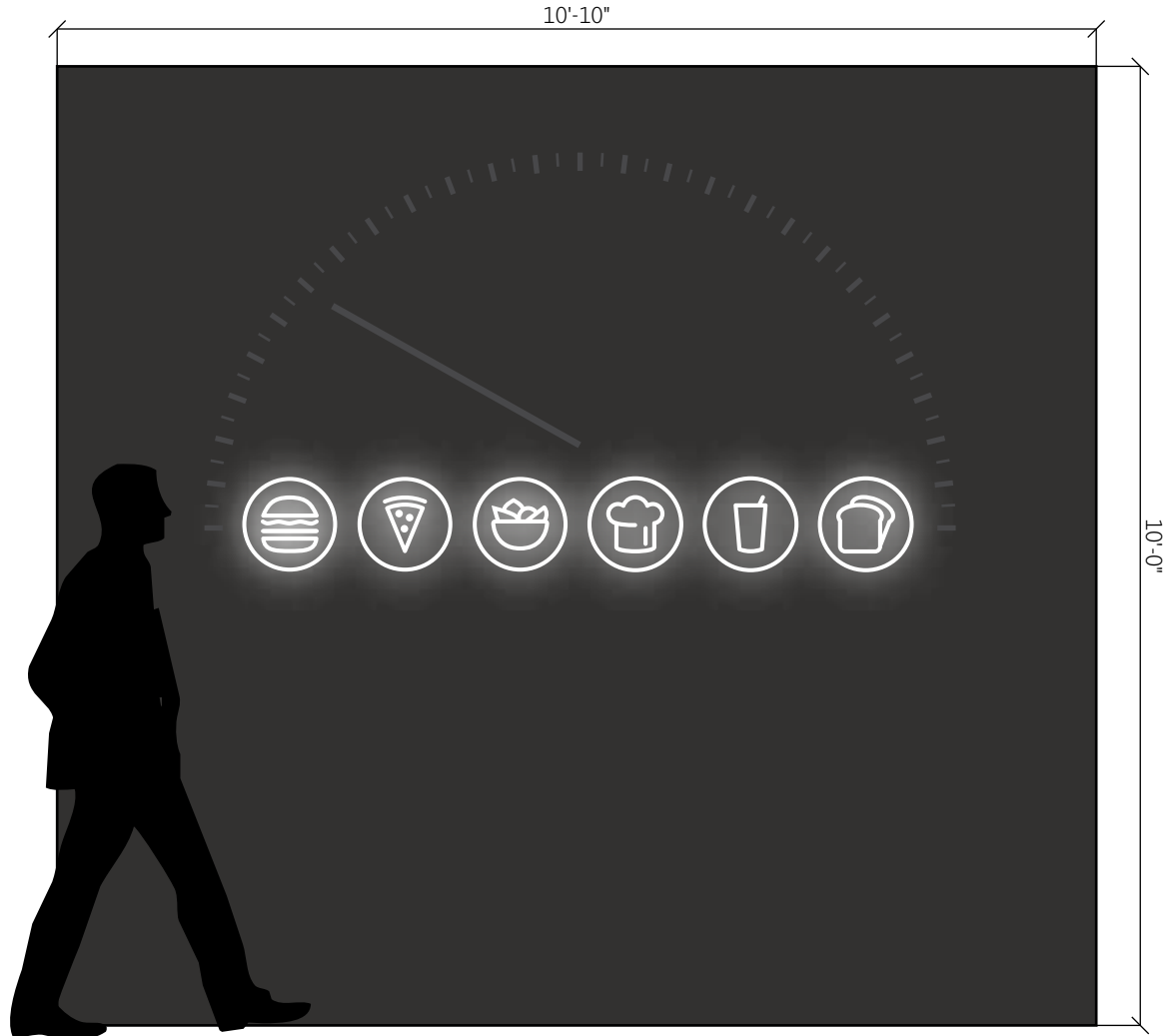
1 ELEVATION - THE SERVERY IDENTITY 1/2"=1'-0"
