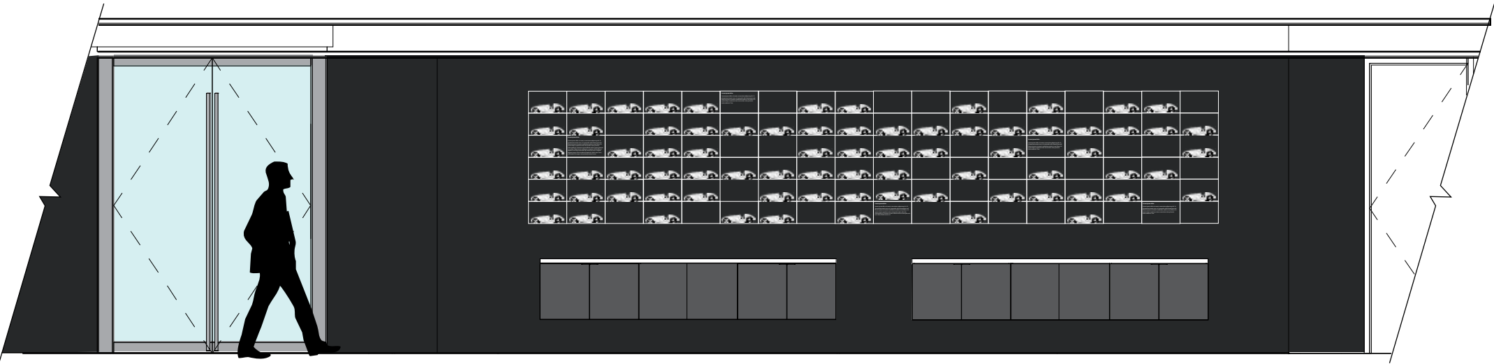
1 ELEVATION - CONFERENCE EXHIBIT WALL 1/4"=1'-0"
