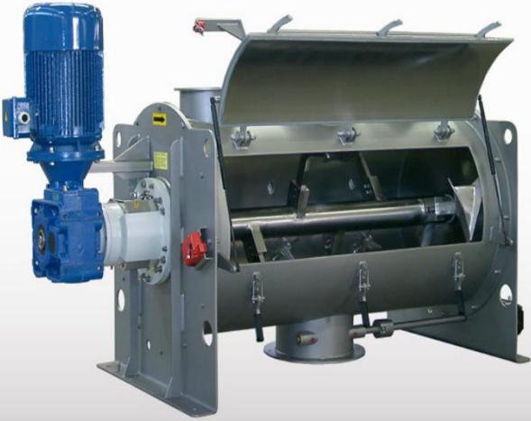
Plough Shear Mixer
