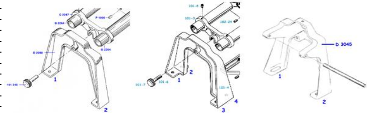
Headrest = 2 Bolt 4 Bolt or J for Jointer
