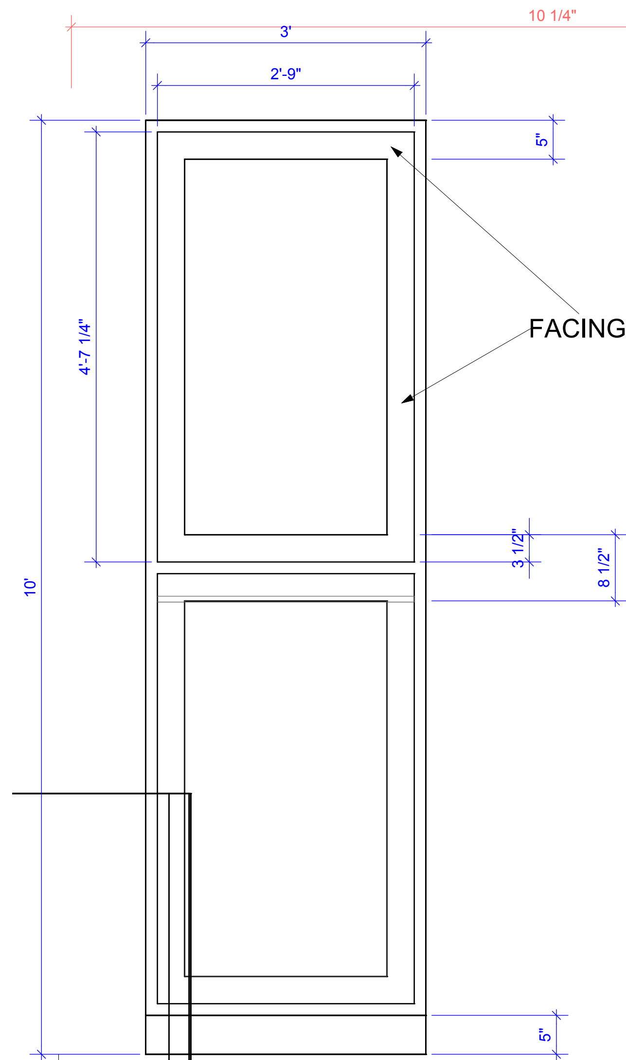
A 5 Trophy Case Front View Scale: 1" = 1'-0"
