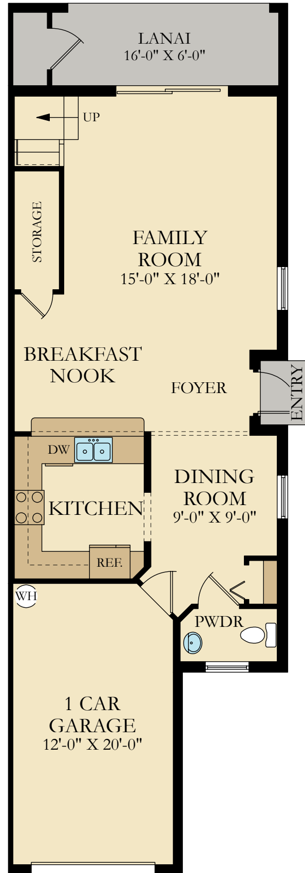
FIRST FLOOR
