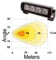
20" FLOOD BEAM
