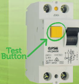
Safety Switch
