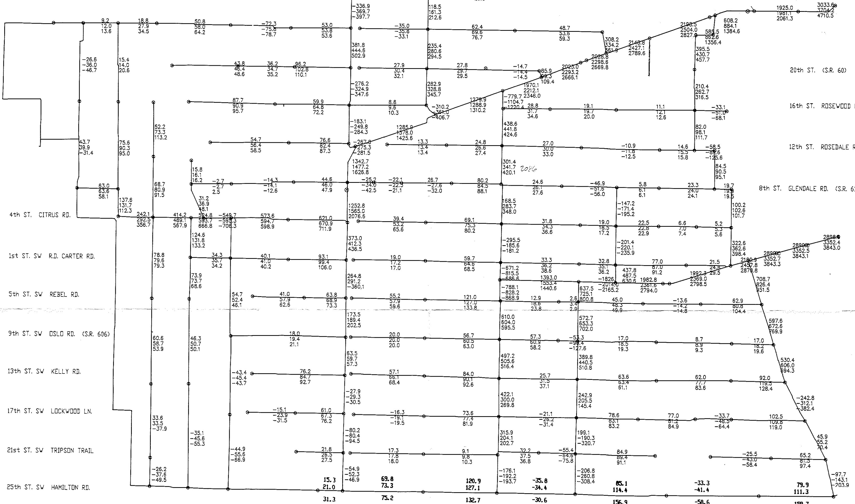
DESIGN STORM FLOWS INDIAN RIVER FARMS WATER CONTROL DISTRICT PROJ. NO. 1920.01 FIGURE 6.2 WILLIAMS HATFIELD & STONER, INC. CARTER ASSOC., INC.
