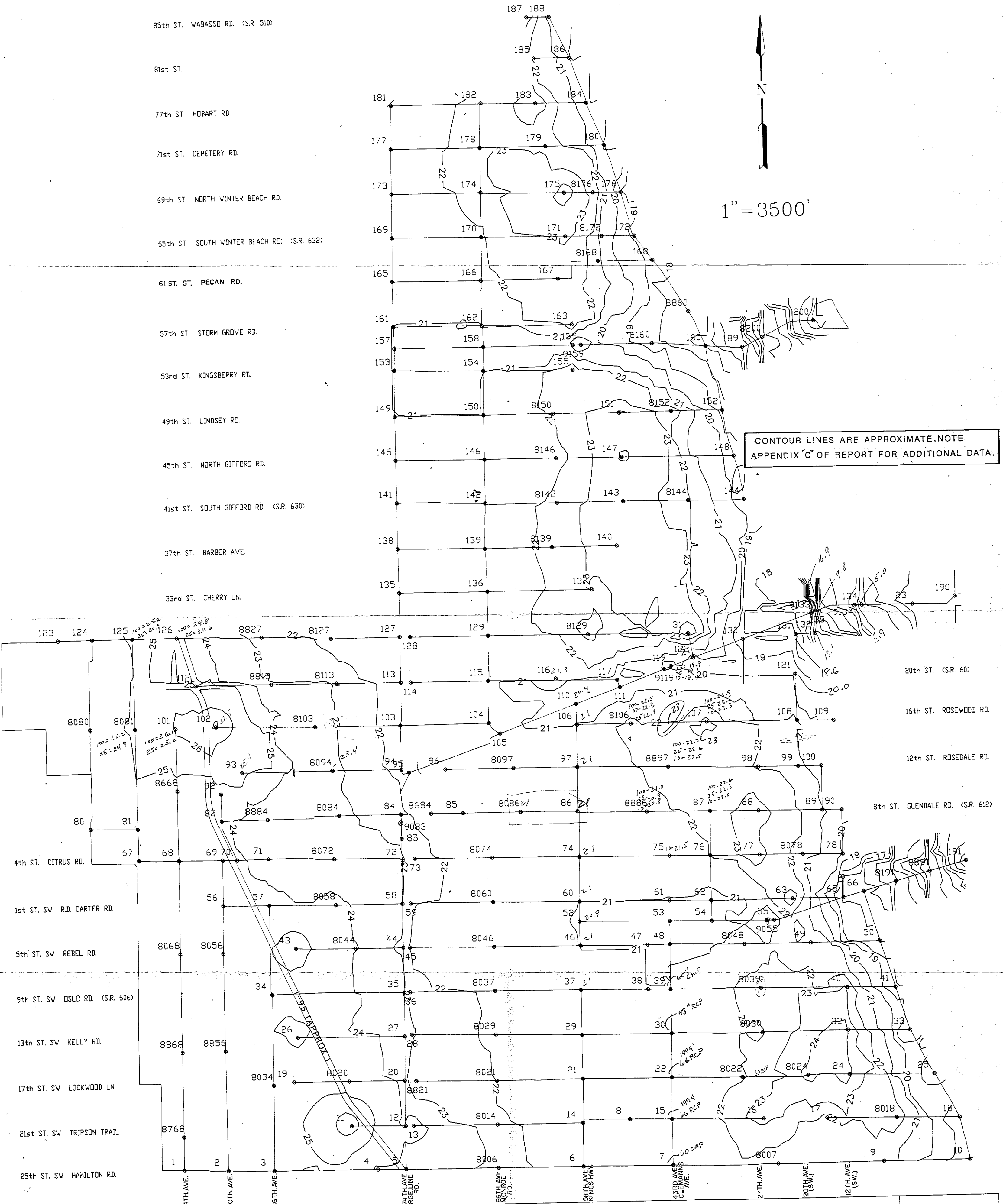
100 YEAR STORM CANAL ELEVATIONS INDIAN RIVER FARMS WATER CONTROL DISTRICT PROJ. NO. 1920.01
