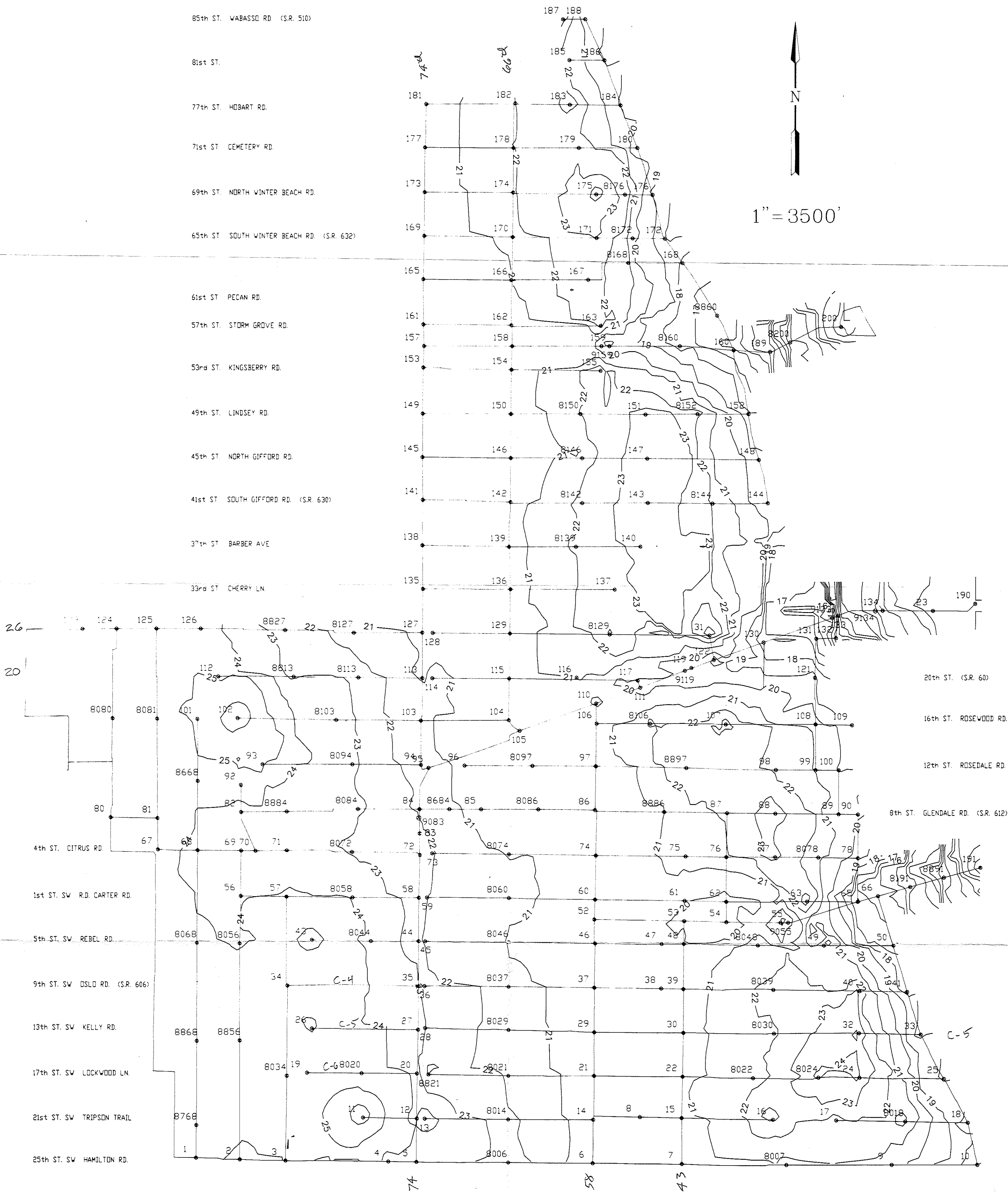
25 YEAR STORM CANAL ELEVATIONS INDIAN RIVER FARMS WATER CONTROL DISTRICT PROJ. NO. 1920.01
