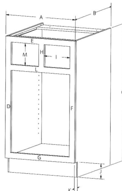
252 | Base Double Drawer
