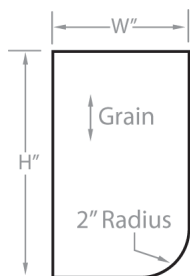
Round Corner Shelf Right*
