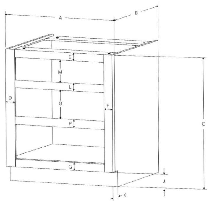
319 | Tree Drawer Base
