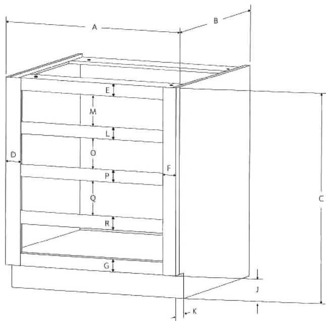
320 | Four Drawer Base
