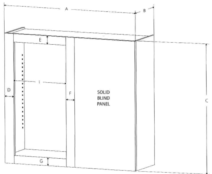
314 | 313 | Blind Corner Right Wall
