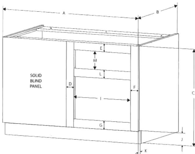
323 | 324 | Blind Corner Left Base Cabinet
