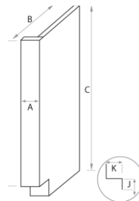
256 | Base End Panel
