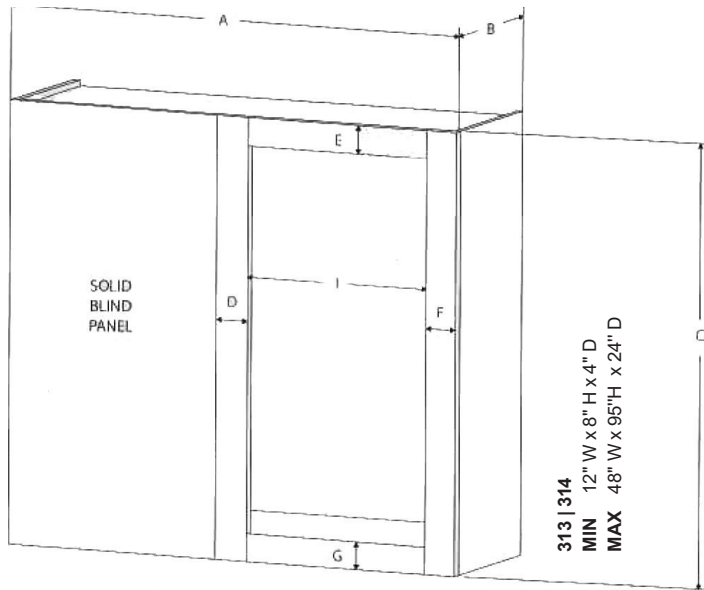
313 | 314 | Blind Corner Left Wall
