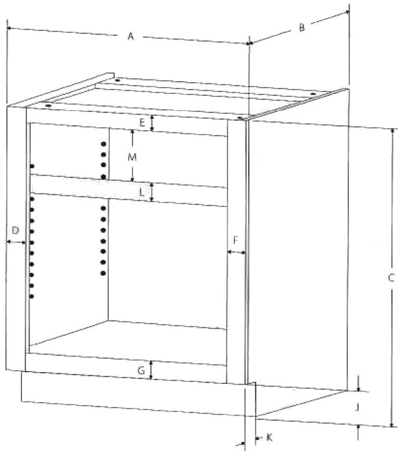
316 | Single Door Base
