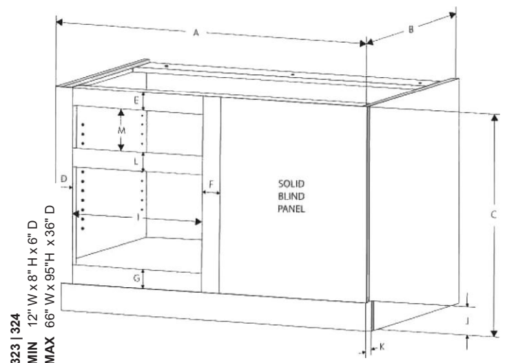
324 | 323 | Blind Corner Right Base Cabinet
