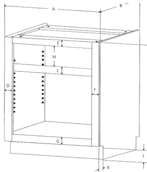
529 | Base Toe Kick Front And Back
