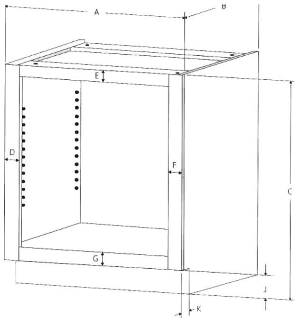
318 | Full Height Base
