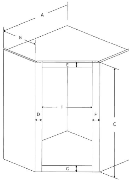
315 | Diagonal Corner Wall
