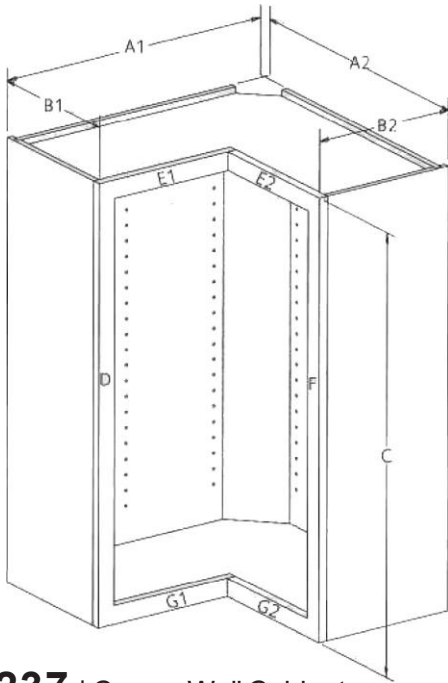
237 | Corner Wall Cabinet
