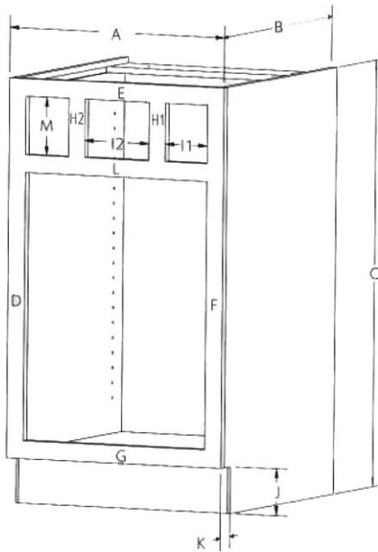
253 | Vanity Three Drawer
