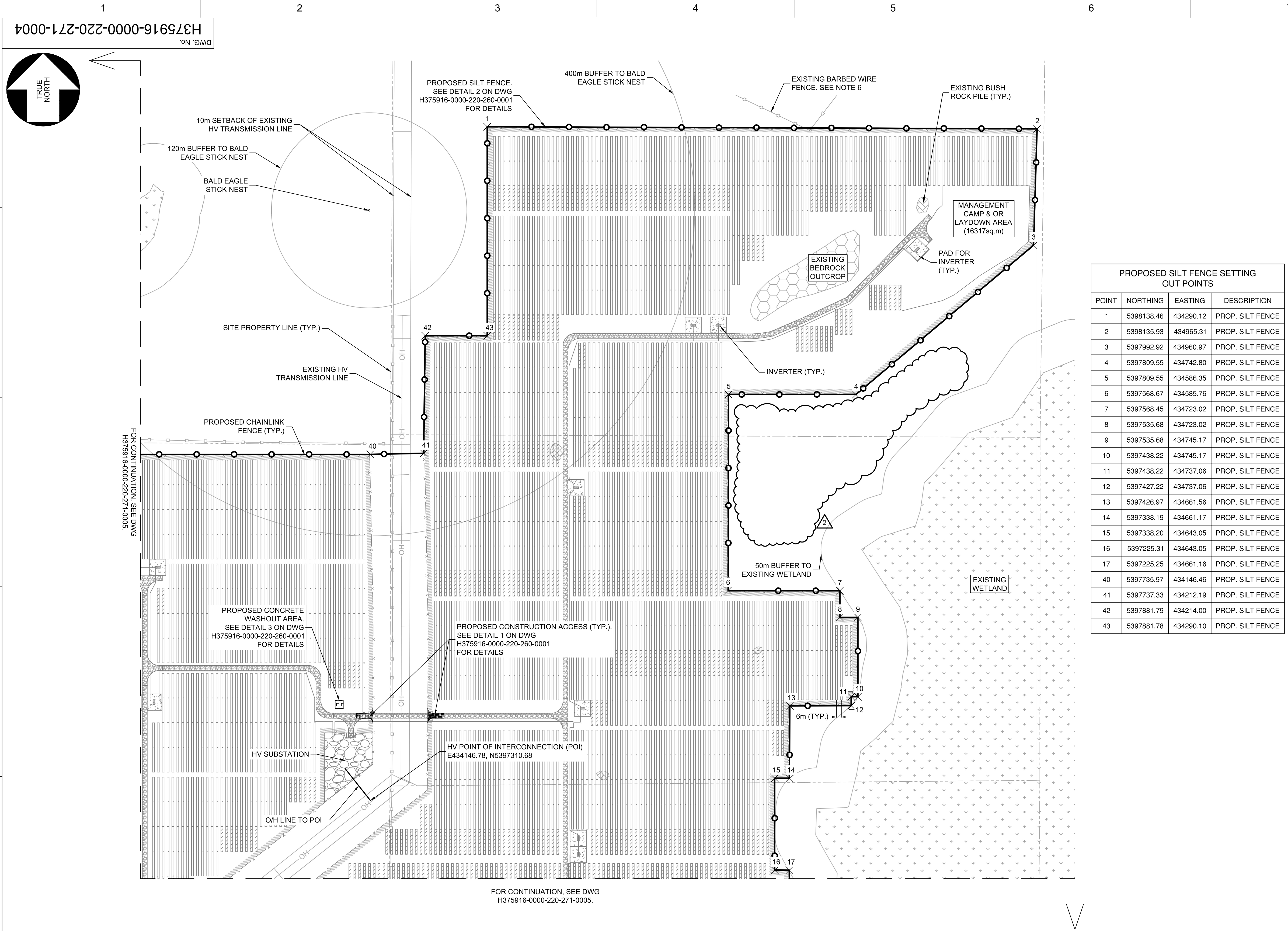
EROSION & SEDIMENT CONTROL (ESC) PLAN 1 SCALE 1:2,500
