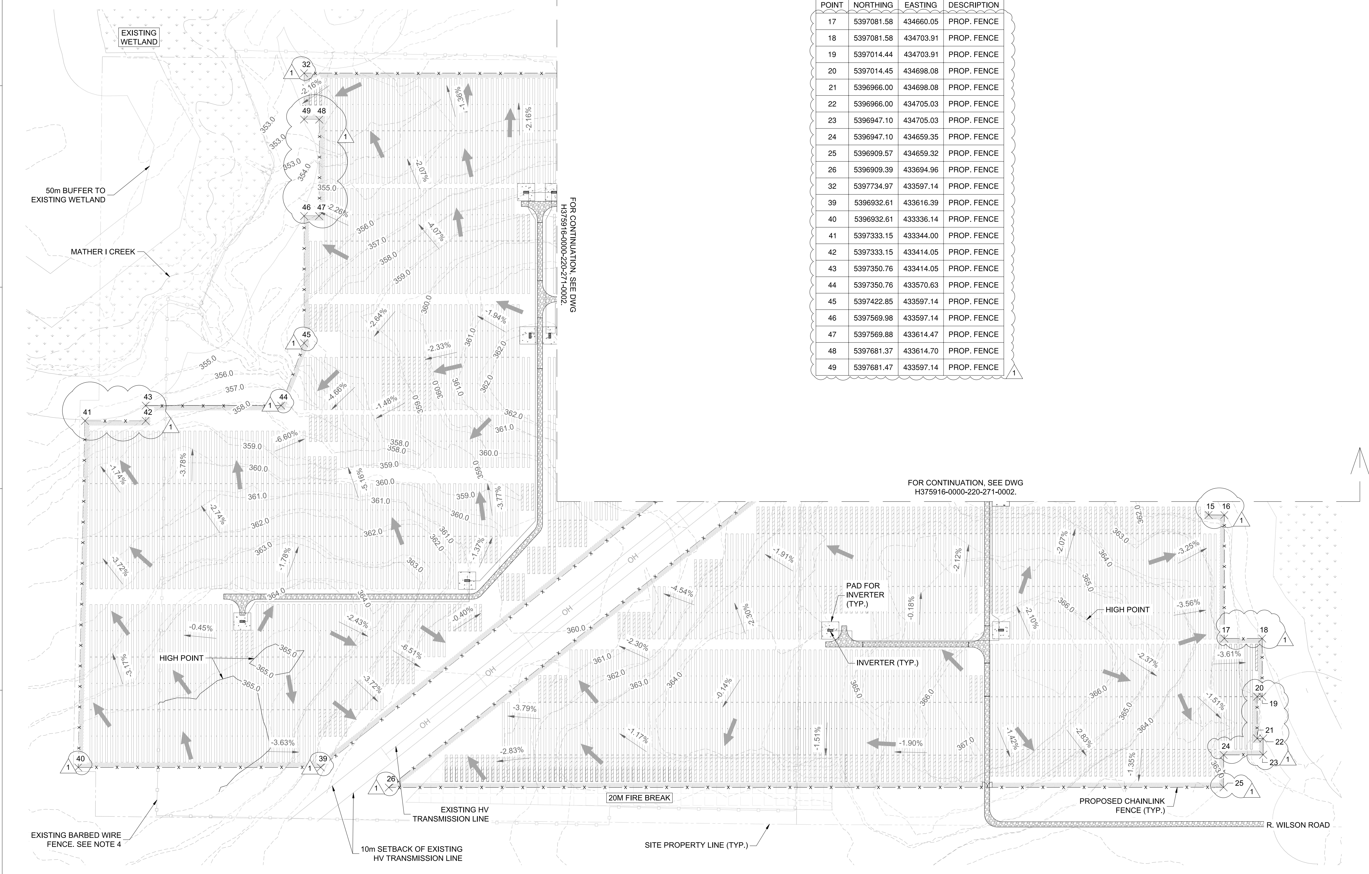
PROPOSED GRADING & DRAINAGE PLAN 2 SCALE 1:2,500
