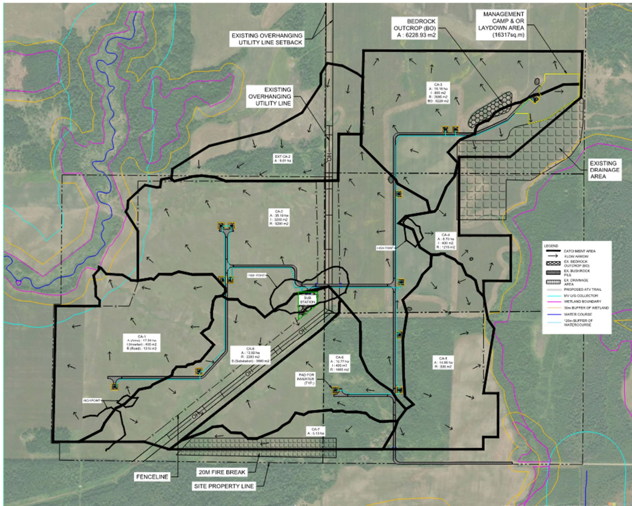
Figure 3-1: Catchment Area for the Proposed Condition
