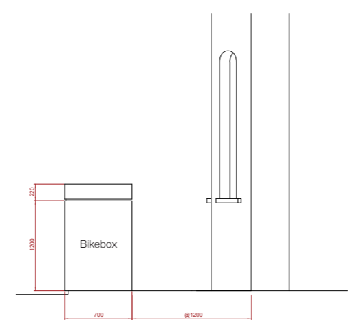
Elevation side view from step
