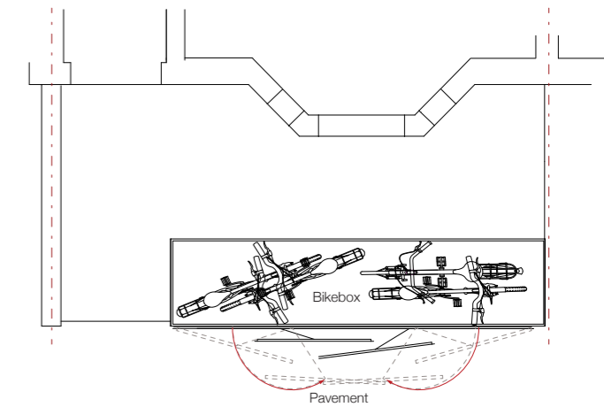
General Plan Opening pavement side
