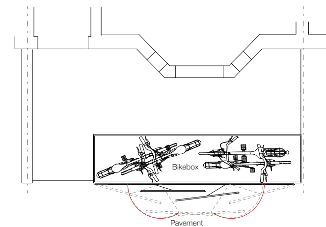
General Plan Opening pavement side
