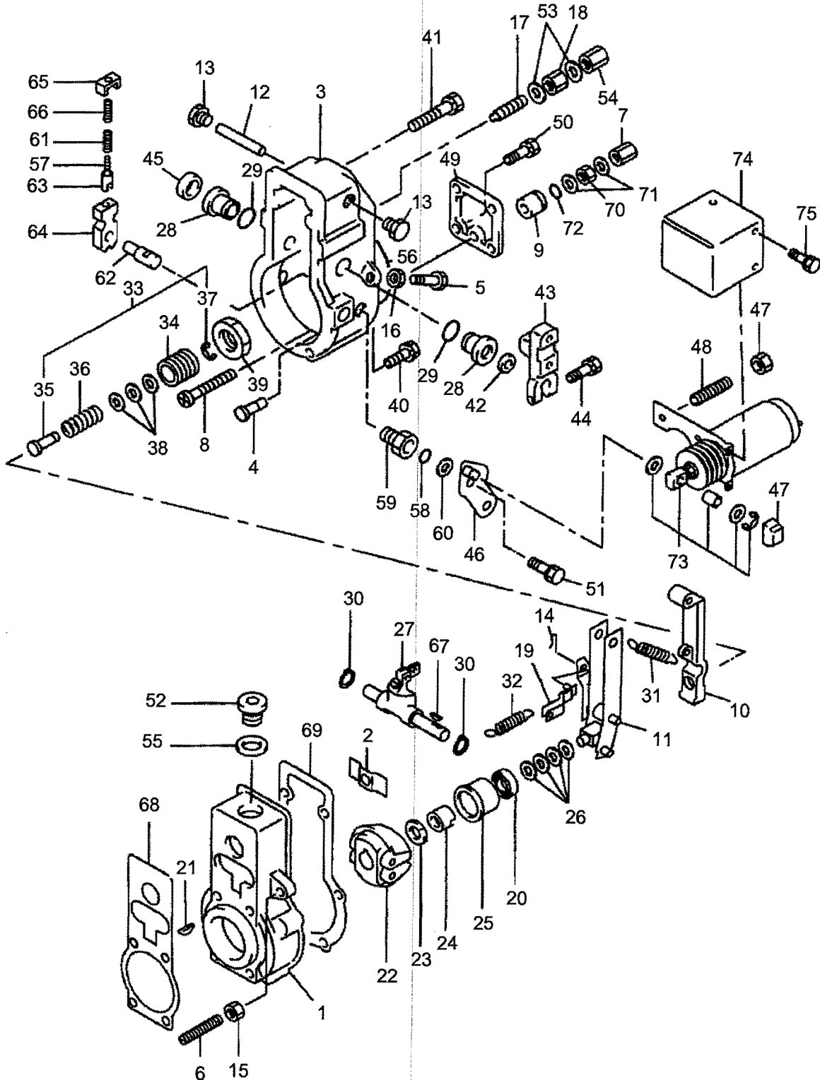
GOVERNOR (INJECTION PUMP, 470 DTC)
