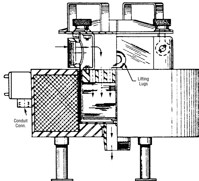
Figure 1 - General schematic of 10-15, 25-15 and 50-15 model magnetic filters with convection cooling.
