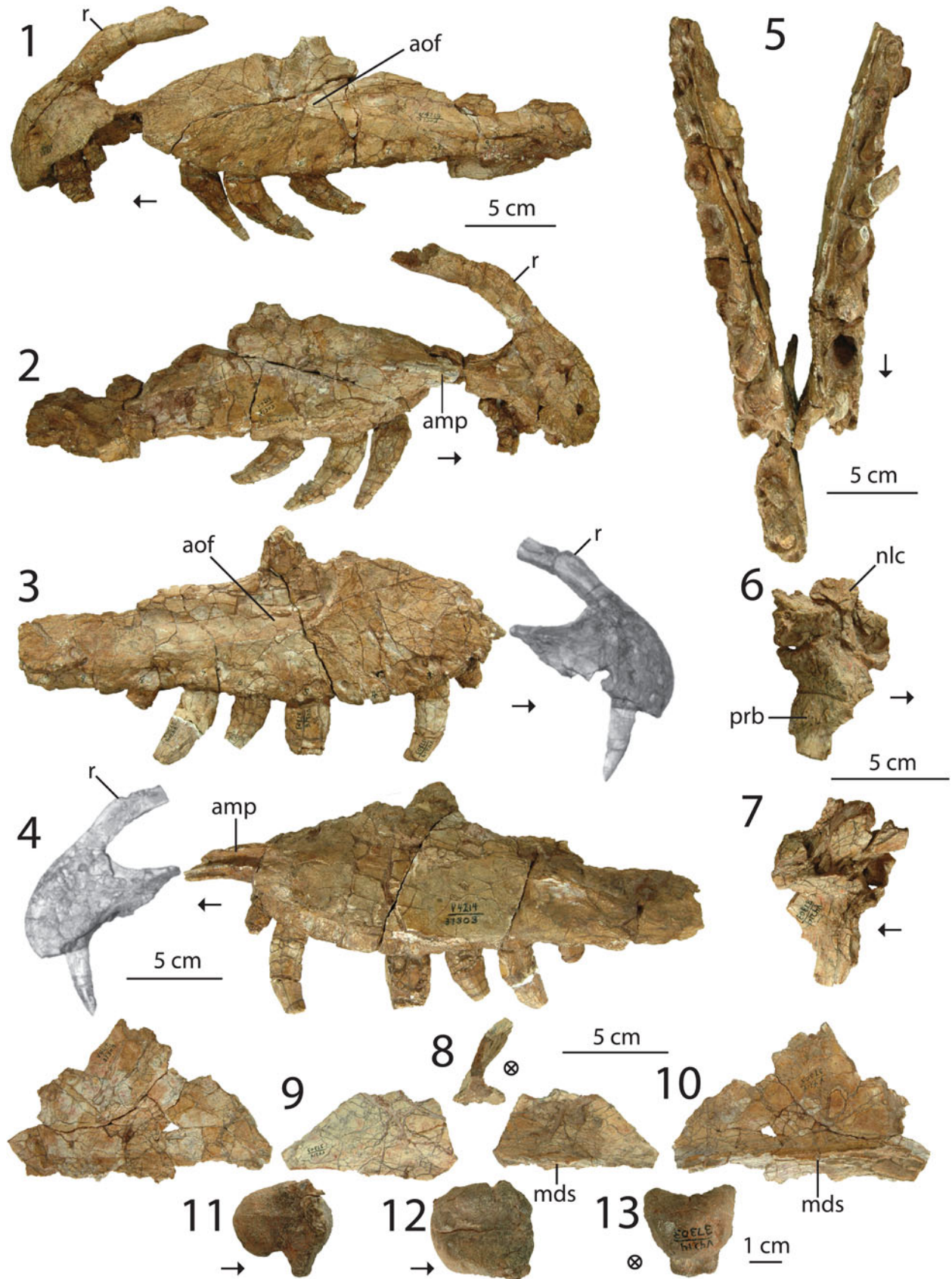
Figure 26. Dilophosaurus wetherilli paratype specimen (UCMP 37303): (1, 2, 5) articulated left maxilla and premaxilla, (3–7) right maxilla and premaxilla, (6, 7) right lacrimal, (8–10) two pieces of the nasolacrimal crests, and (11–13) basioccipital in (1, 3, 6, 9, 11) lateral, (2, 4, 7, 10) medial, (12) dorsal, (5) ventral, and (8, 13) posterior view. Arrows point in anterior direction. amp = anteromedial process; aof = antorbital fossa; mds = midline suture; nlc = nasolacrimal crest; prb = preorbital boss; r = ridge.
