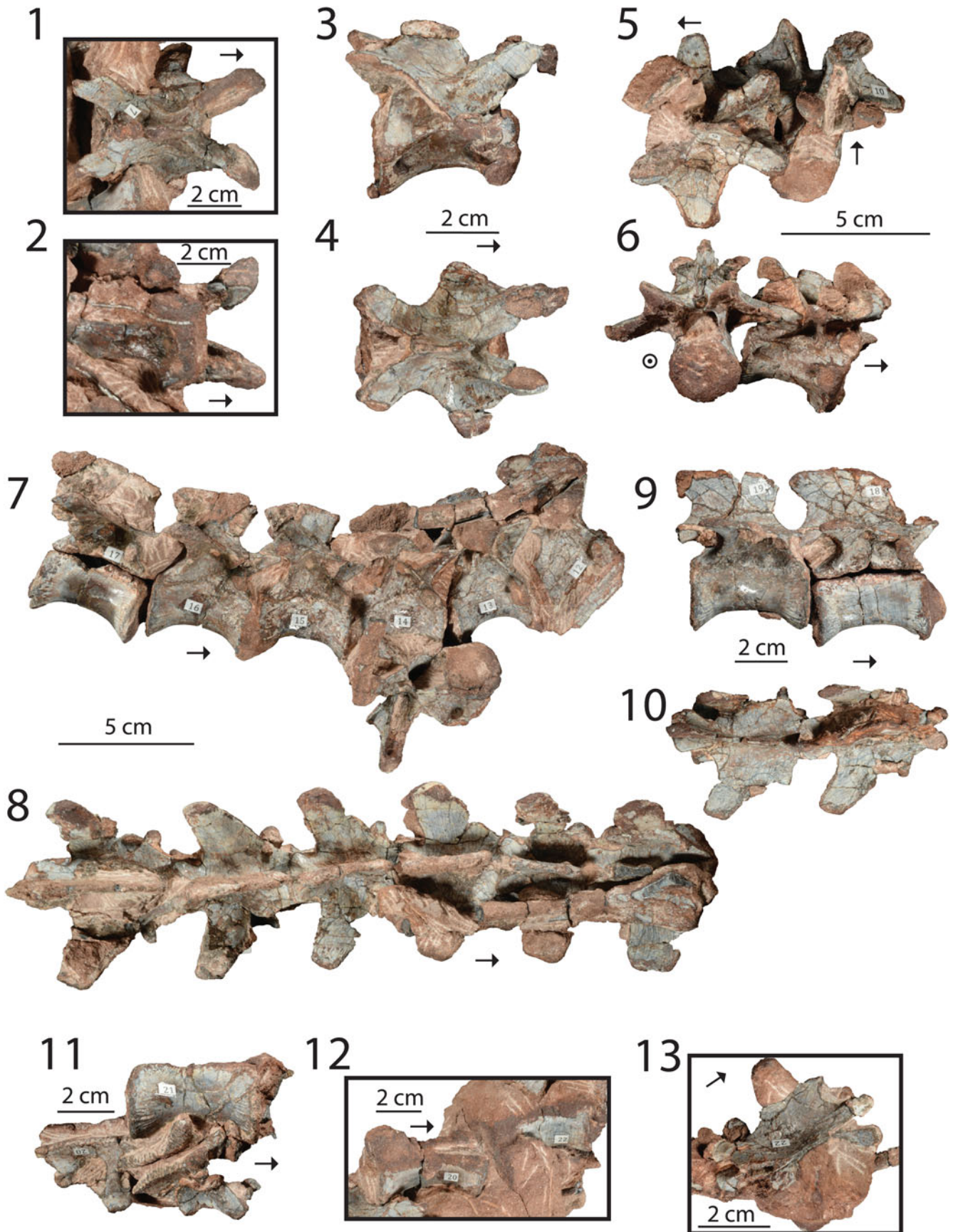
Figure 60. Dilophosaurus wetherilli referred specimen (TMM 47006-1): (1, 2) seventh cervical, (3, 4) eighth cervical, (5, 6) ninth and tenth cervical, (7, 8) 11th through 17th vertebra, (9, 10) 18th and 19th vertebra, (11) 20th neural arch and 21st vertebra, (12) 20th and 22nd centra, and (13) 22nd neural arch in (1, 4, 5, 8, 10, 13) dorsal, (2) ventral, (3, 6, 7, 9, 11, 12) lateral, and (6) posterior view. Arrows point in anterior direction.
