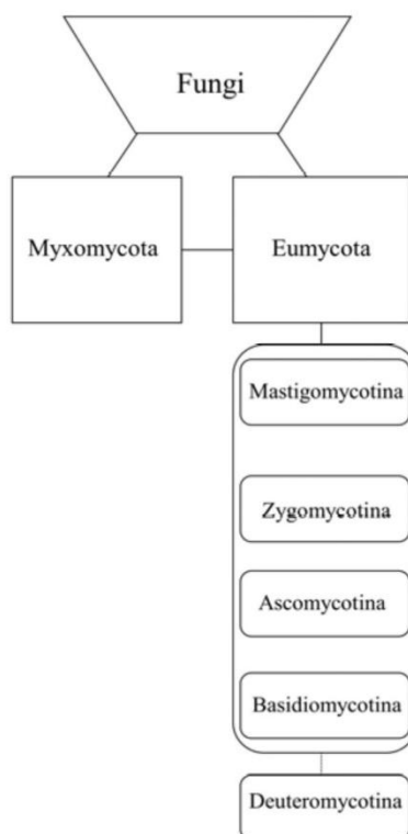
Fig. 2 - Traditional fungal classification, as outlined by Ainsworth et al. (1973), grouped fungi and fungi-like organisms under the Kingdom Plantae, dividing them into Myxomycota (slime molds) and Eumycota (true fungi). The Eumycota included the following groups: Mastigomycotina, Zygomycotina, Ascomycotina, Basidiomycotina, and Deuteromycotina, based on morphological and reproductive characteristics (Source: Shenoy et al. (2007)/Fungal Diversity/CC BY)
