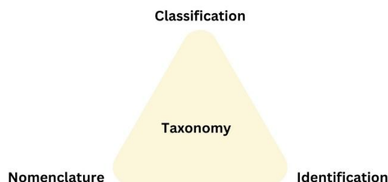
Fig. 1 - The three foundational components of taxonomy—identification, nomenclature, and classification—are illustrated as integral elements forming the basis of taxonomic practice. Together, they facilitate the scientific understanding and organisation of biological diversity based on evolutionary relationships.
