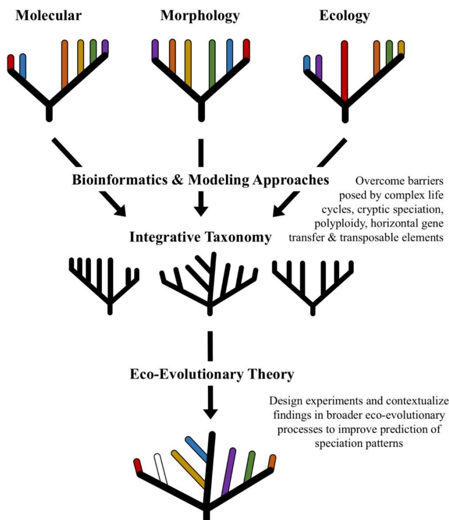
Fig. 4 - Integrative taxonomic framework combining molecular, morphological, and ecological data through bioinformatic and modeling approaches to address challenges including cryptic speciation, polyploidy, and horizontal gene transfer. This eco-evolutionary approach enhances species boundary resolution by incorporating evolutionary context (Source: Stengel et al. (2022)/Frontiers in Microbiology/CC BY)
