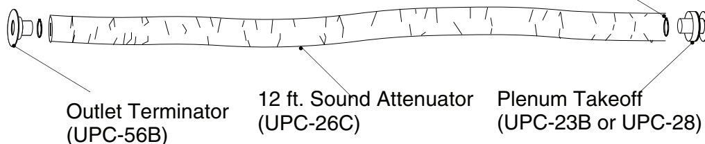
Figure 1. Plenum Takeoff
