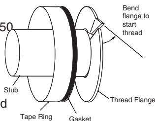
Figure 2. Spin-In Takeoff 1" Pre Insulate Duct
