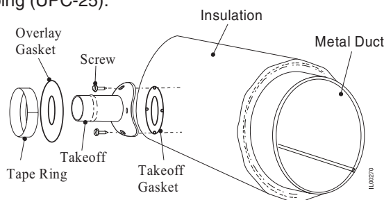
Figure 3. Metal Takeoff Installation
