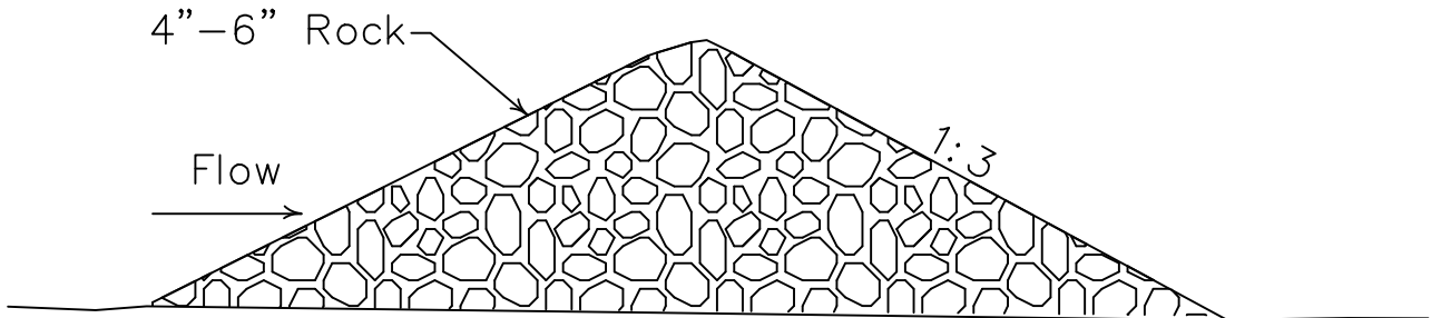
ROCK CHECK DAM CROSS-SECTION
