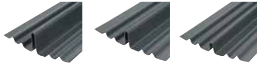
105mm upstand 80mm upstand 55mm upstand
