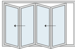
4 SHUTTER
