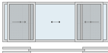
3 TRACK - 3 SHUTTER + 2 MESH SHUTTER
