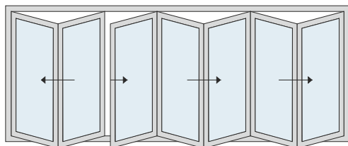
2 SHUTTER + 5 SHUTTER
