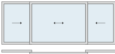
2 TRACK - 3 SHUTTER (X-2X-X)
