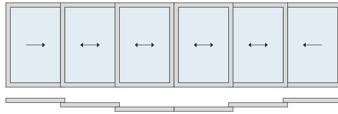
3 TRACK - 6 SHUTTER
