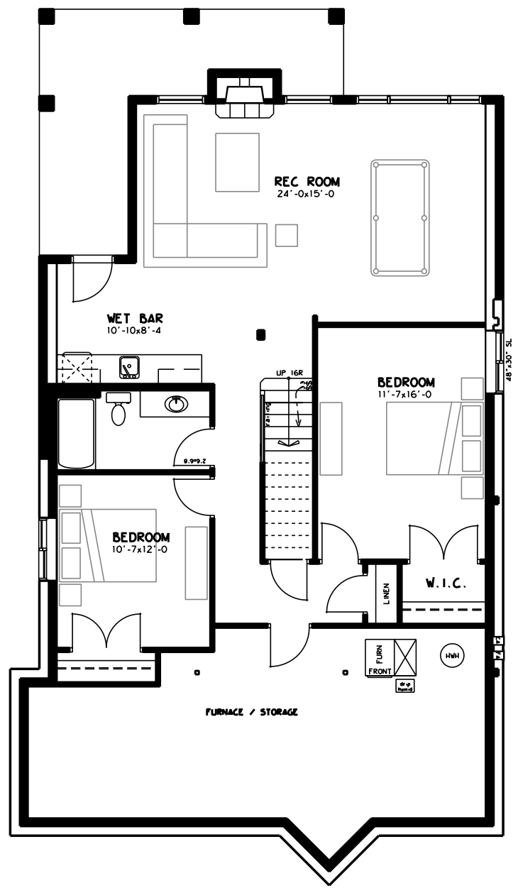
Basement Development 1080 SQ.FT.
