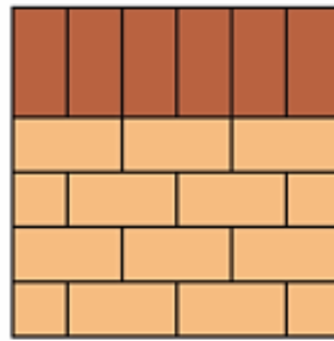
Stretcher Bond with contrasting header
