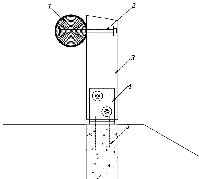
Figure 10: Traffic barrier with timber rail
