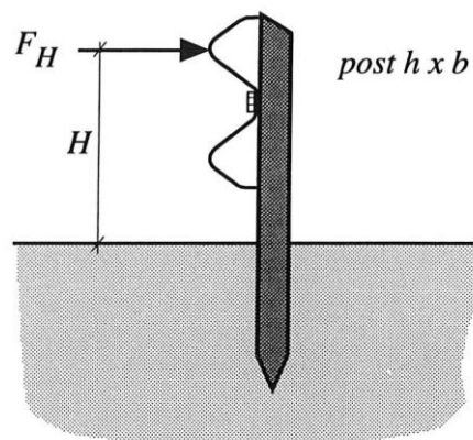
Figure 9: Traffic barrier.
