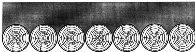
Figure 1: Simple contiguous pole wall (in plan showing retained material).
