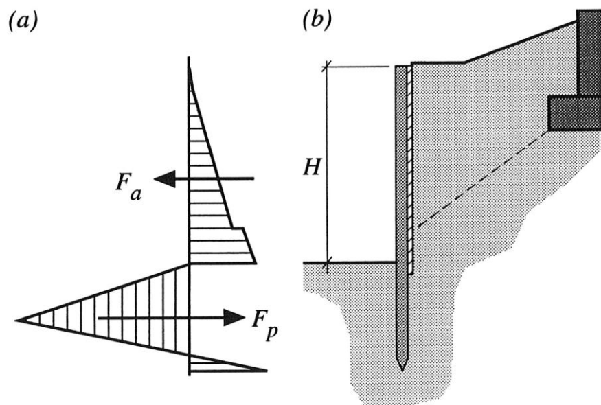
Figure 5: Pressure diagram and loads for a retaining wall. F_a = active force and F_p = passive force.
