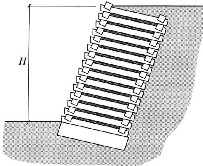
Figure 6: Typical crib retaining wall
