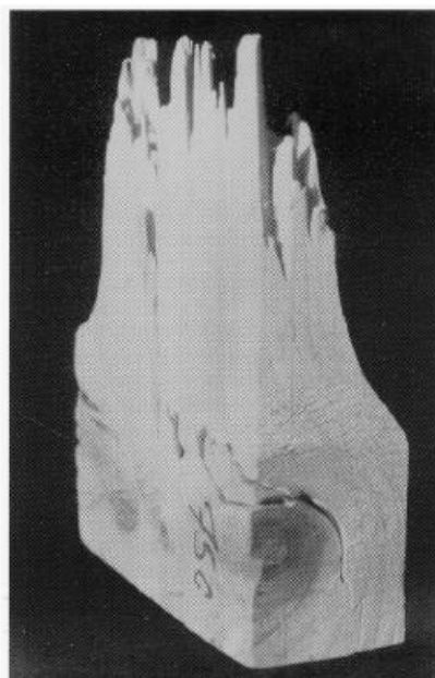
Figure 7: Tension failure of a spruce board caused by fibre inclination around a knot.
