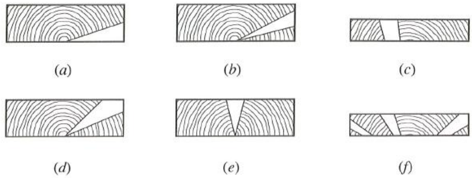
Figure 10: Knots are termed according to their appearance at the surface of the timber; (a) spike knot; (b) narrow face knot; (c) through knot; (d) arris knot; (e) wide face knot; (f) knot cluster.
