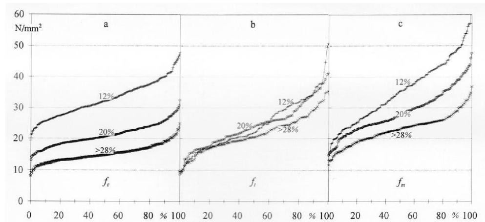
Figure 17: Strength ( N/mm^2 ) against percentile for matched samples of spruce ( Picea abies ) subjected to a: compression, b: tension and c: bending at moisture content levels 12%, 20% and >28%.
