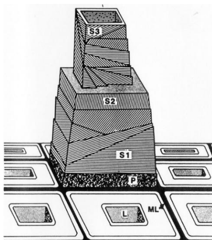
Figure 4: Schematic of the general wall architecture of normal wood fibres.
