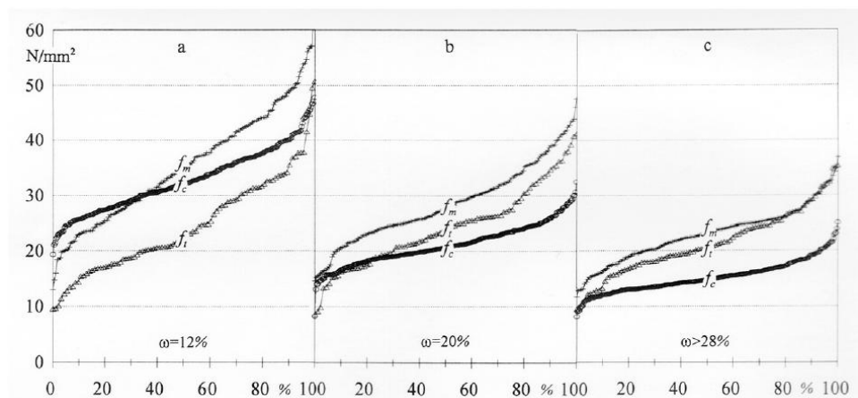
Figure 18: Strength ( N/mm^2 ) against percentile (%) for matched samples of spruce ( Picea abies ). The results shown in Figure 17 have been rearranged to illustrate the interrelationship of compression-, tension- and bending strength at equal moisture content levels.
