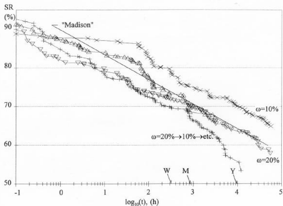
Figure 20: Stress ratio (%) against logarithmic time to failure (hours) for 50 x 100 mm beams of spruce ( Picea abies ) subjected to bending at \sigma = 10\% , ( D = 20\% and at D cycling between 10% and 20%. +: varying moisture content; A: 20% moisture content; x = 10% moisture content. Y = one year. M = one month. W = one week (reproduced after Hoffmeyer, 1990).
