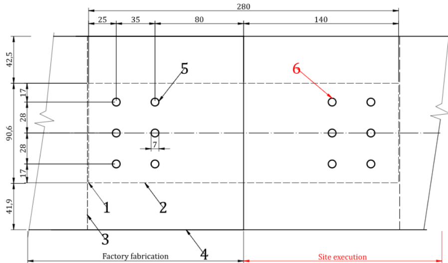
Figure 10: Dowel plate connection
