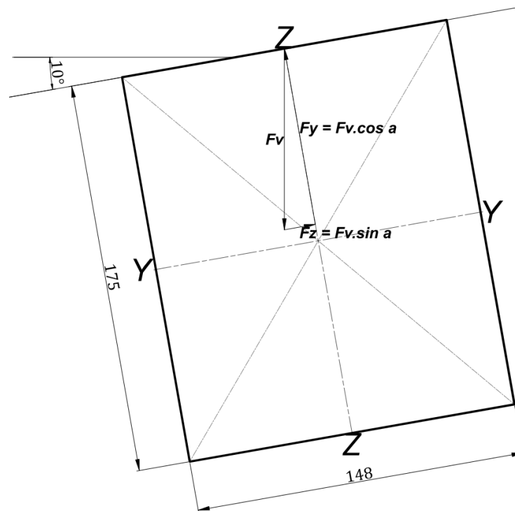
Figure 4: Purlin section configuration
