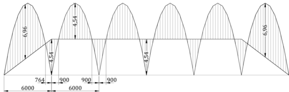
Figure 5: Typical bending moment diagram
