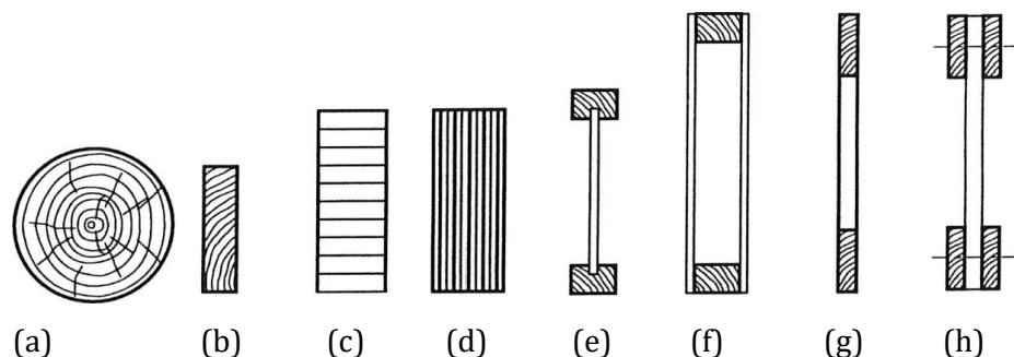
Figure 1; Examples of Purlin sections.
