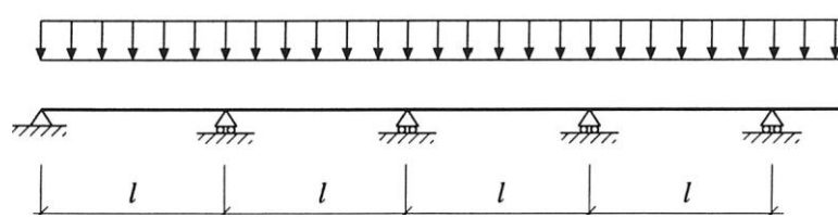
Figure 3: Example purlin.
