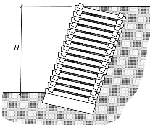
Figure 5 Typical crib retaining wall.
