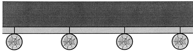
Figure 2 Plan of spaced pole and board wall.
