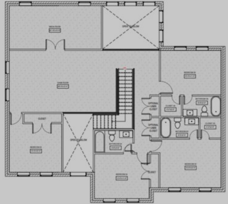
○ SECOND FLOOR 1/28
