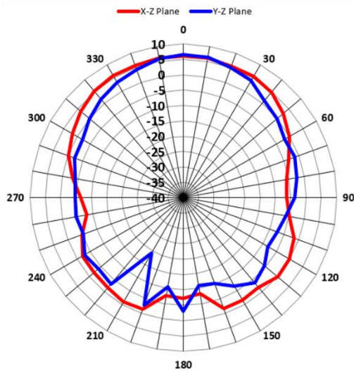
3.5GHz_Vertical
