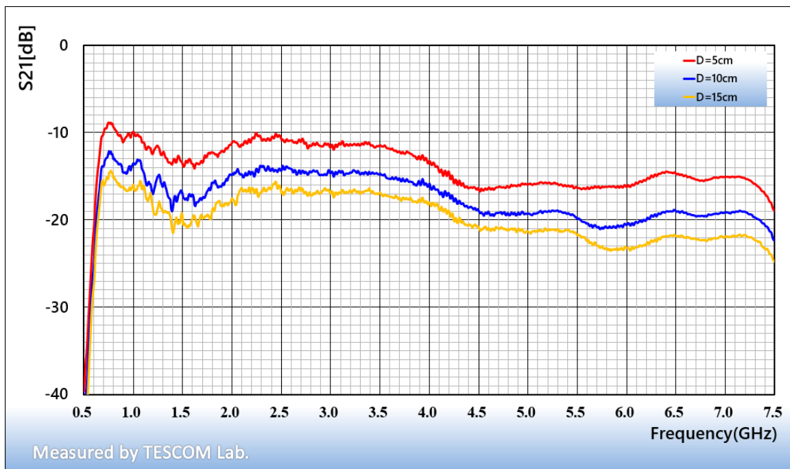
Graph 4. TC-93076A Path-Loss (Vertical)
