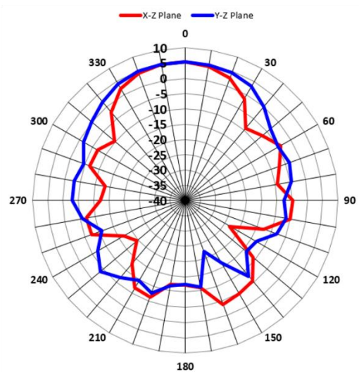
7.0GHz_Vertical
