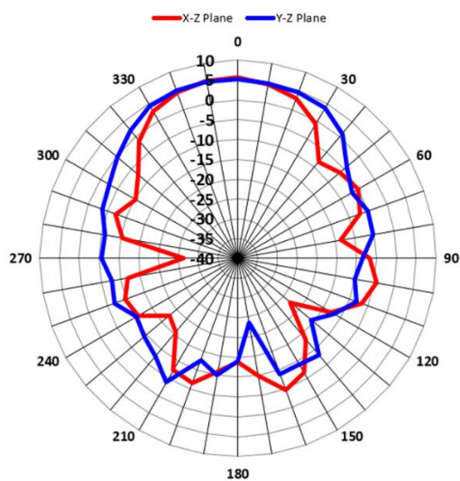
6.5GHz_Vertical
