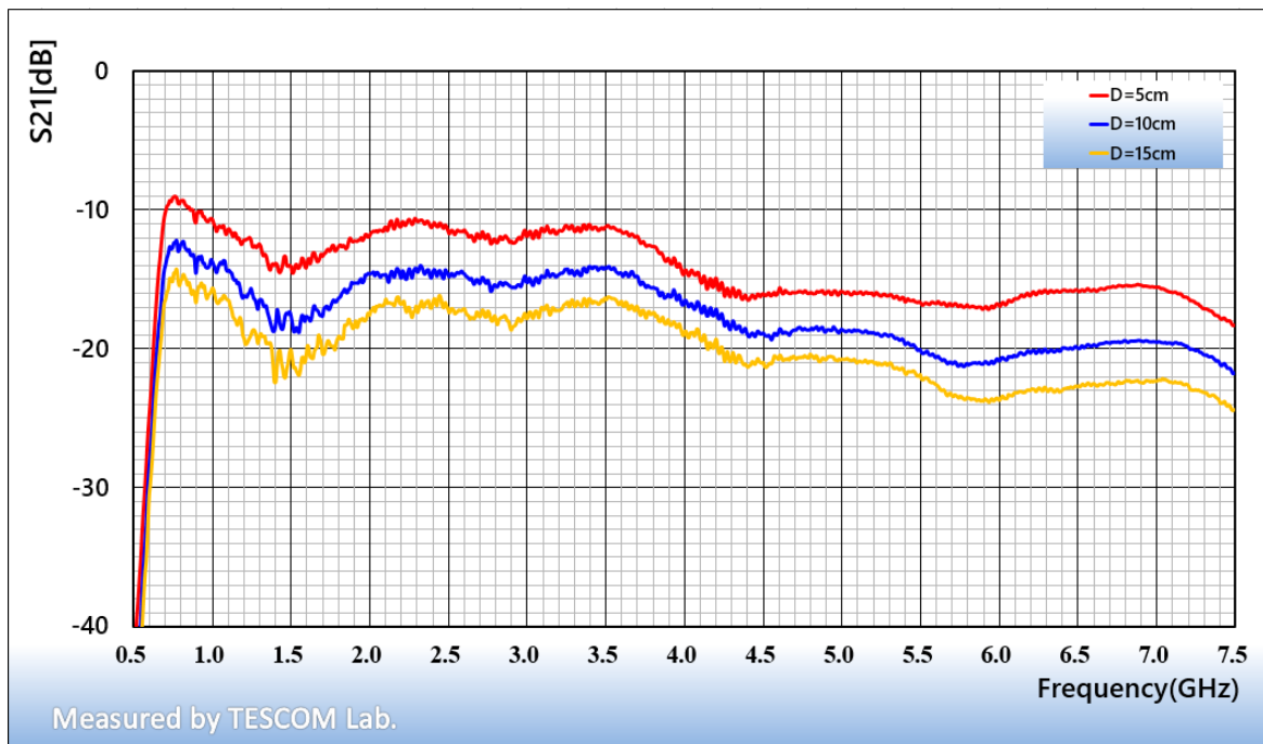
Graph 3. TC-93076A Path-Loss (Horizontal)
