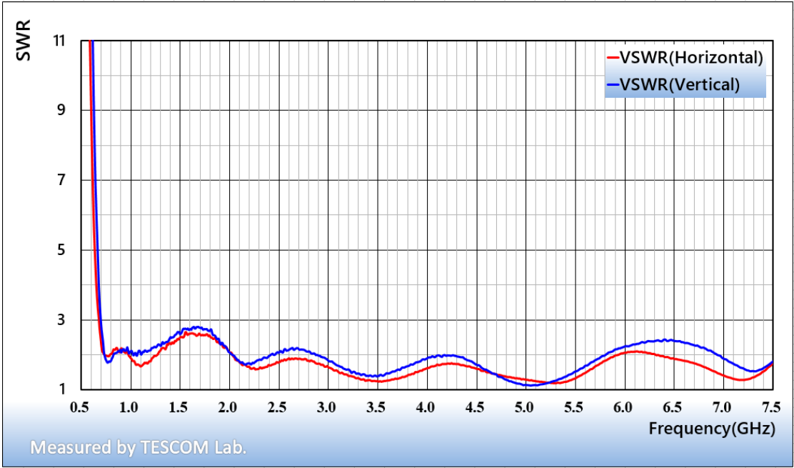
Graph 1. TC-93076A VSWR
