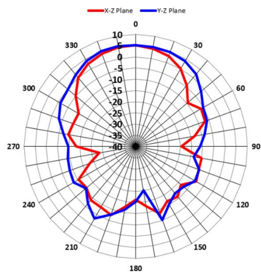
6.0GHz_Vertical
