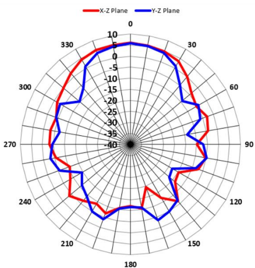
7.0GHz_Horizontal
