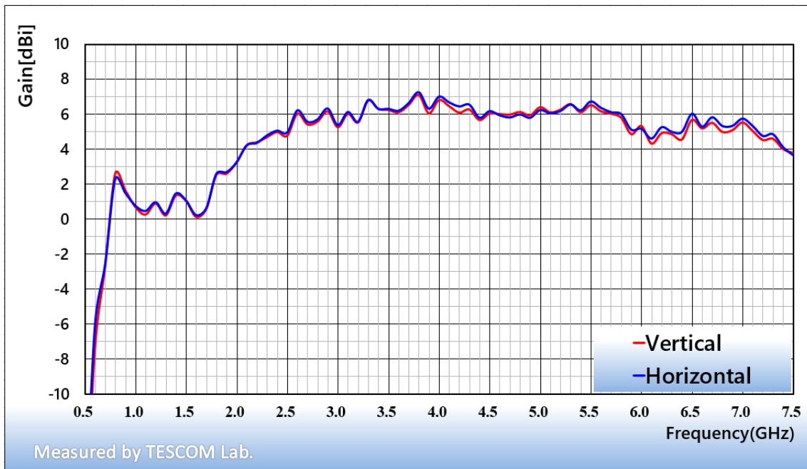
Graph 2. TC-93076A Gain
