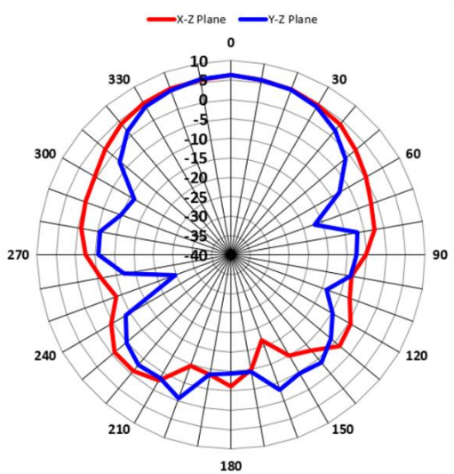
5.0GHz_Horizontal
