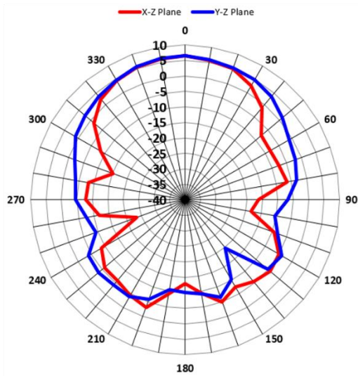
5.5GHz_Vertical
