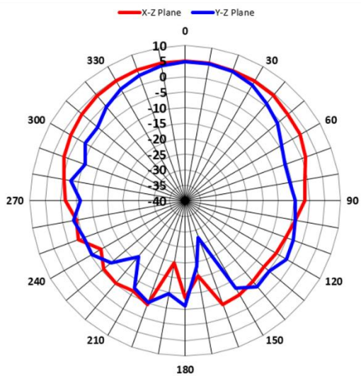
2.4GHz_Vertical
