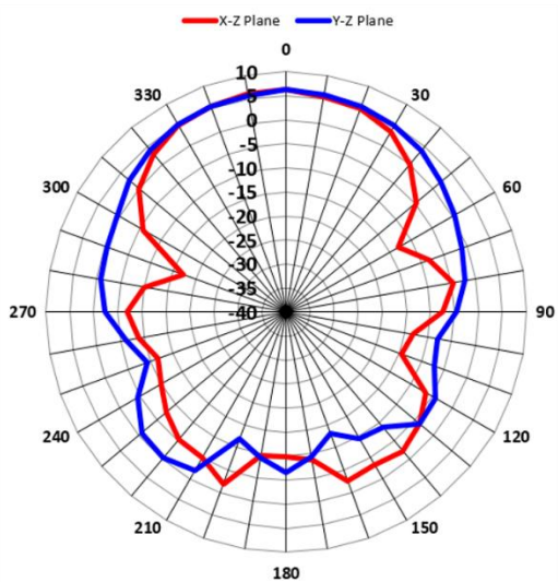
5.0GHz_Vertical
