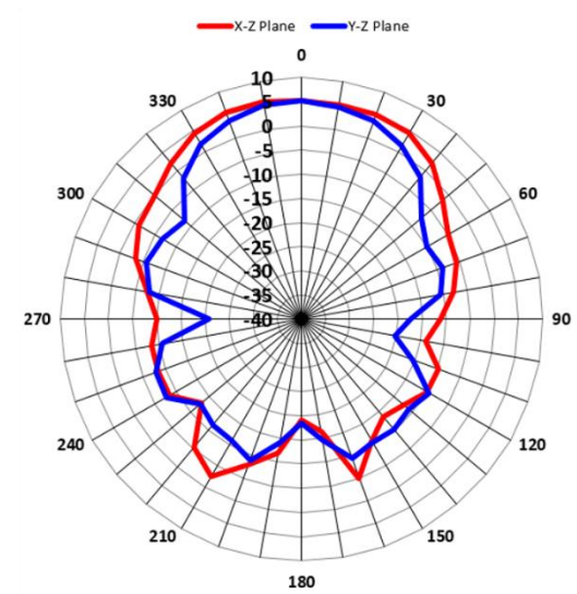
6.0GHz_Horizontal
