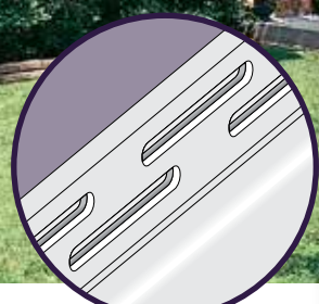
Double staggered nail slots hit a stud every time.
