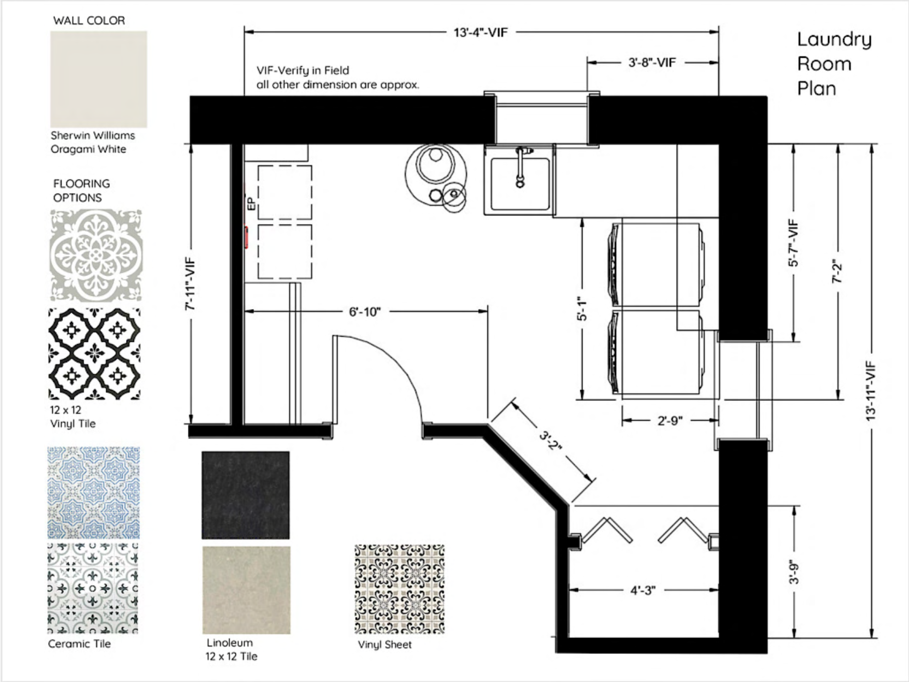
Bowker Laundry Room - Phase 2 Build / FF&E
