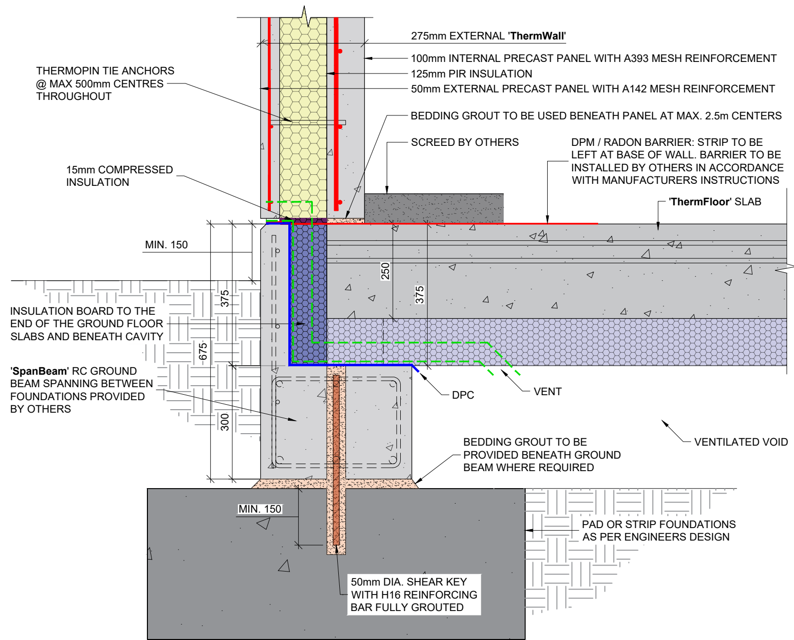
TYPICAL SECTION THROUGH EXTERNAL WALL SUPPORTS SCALE 1:10
