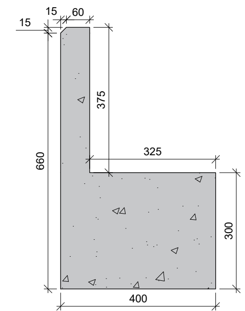
EXTERNAL GROUND BEAM GEOMETRY SCALE 1:10
