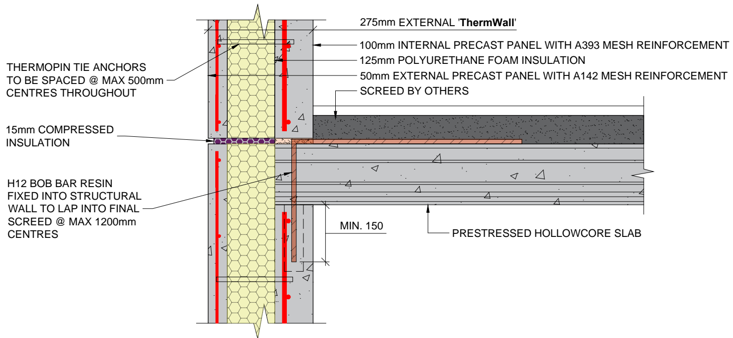
'ThermWall' FIRST FLOOR CONNECTION DETAIL
